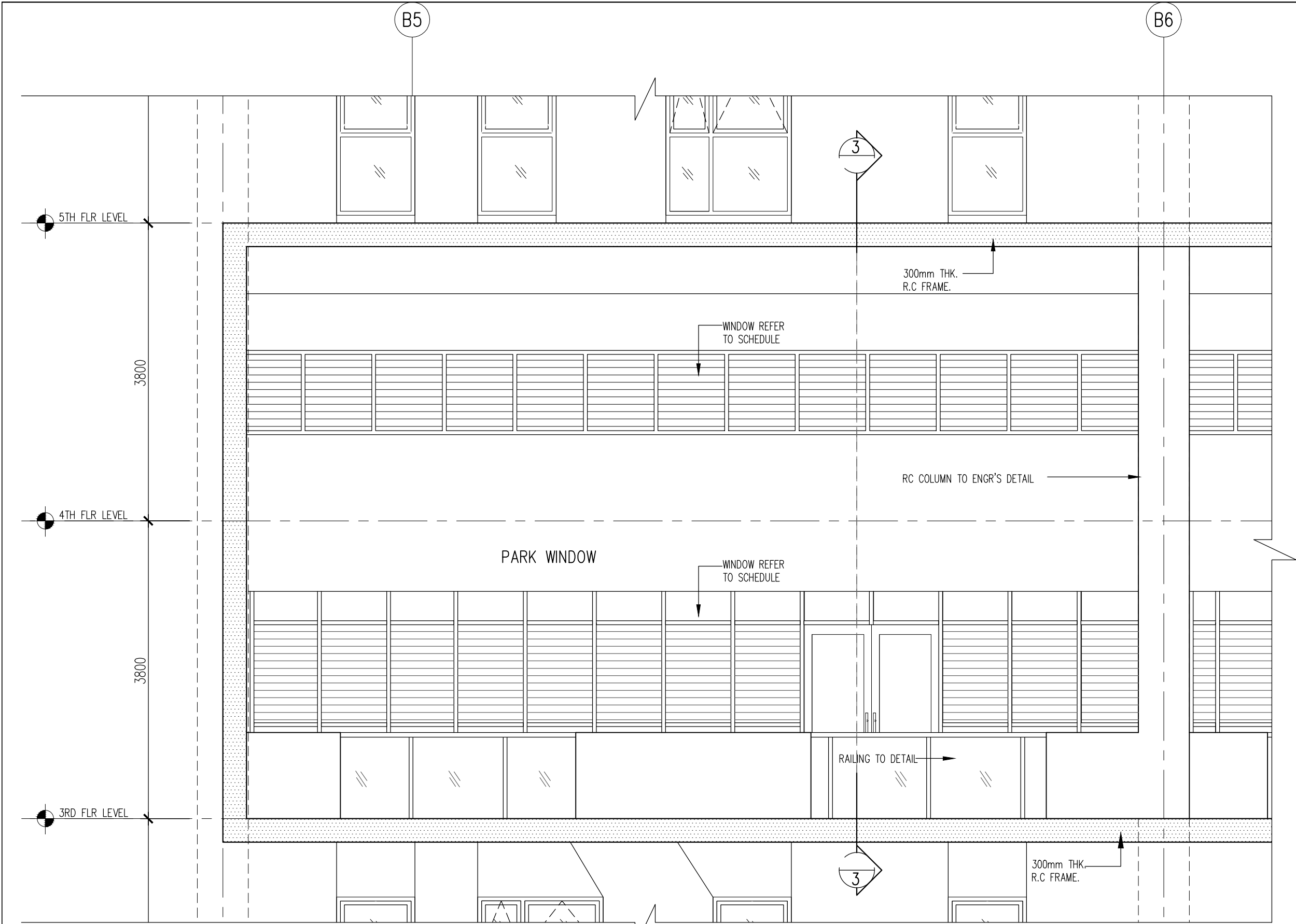
2 ELEVATION SCALE = 1 : 50
