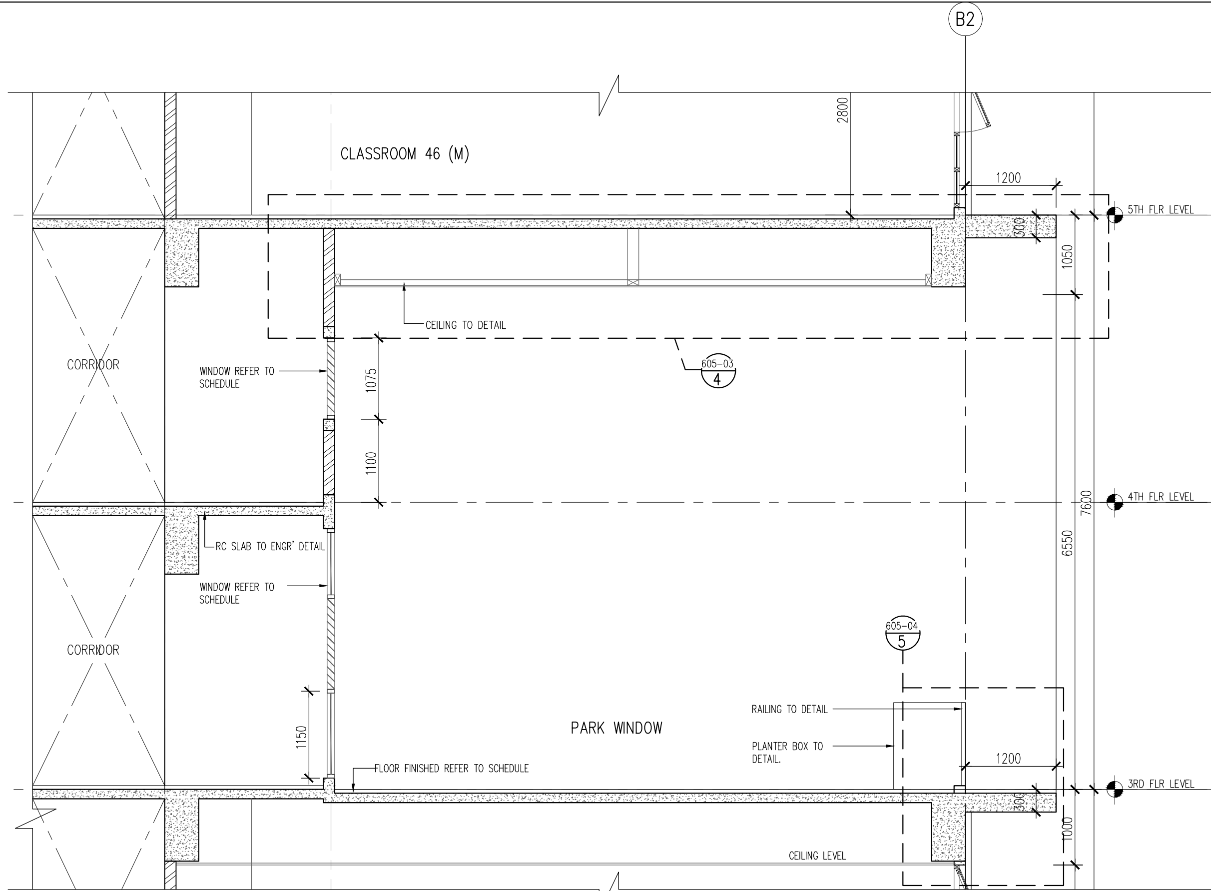
3 SECTION SCALE = 1 : 50
