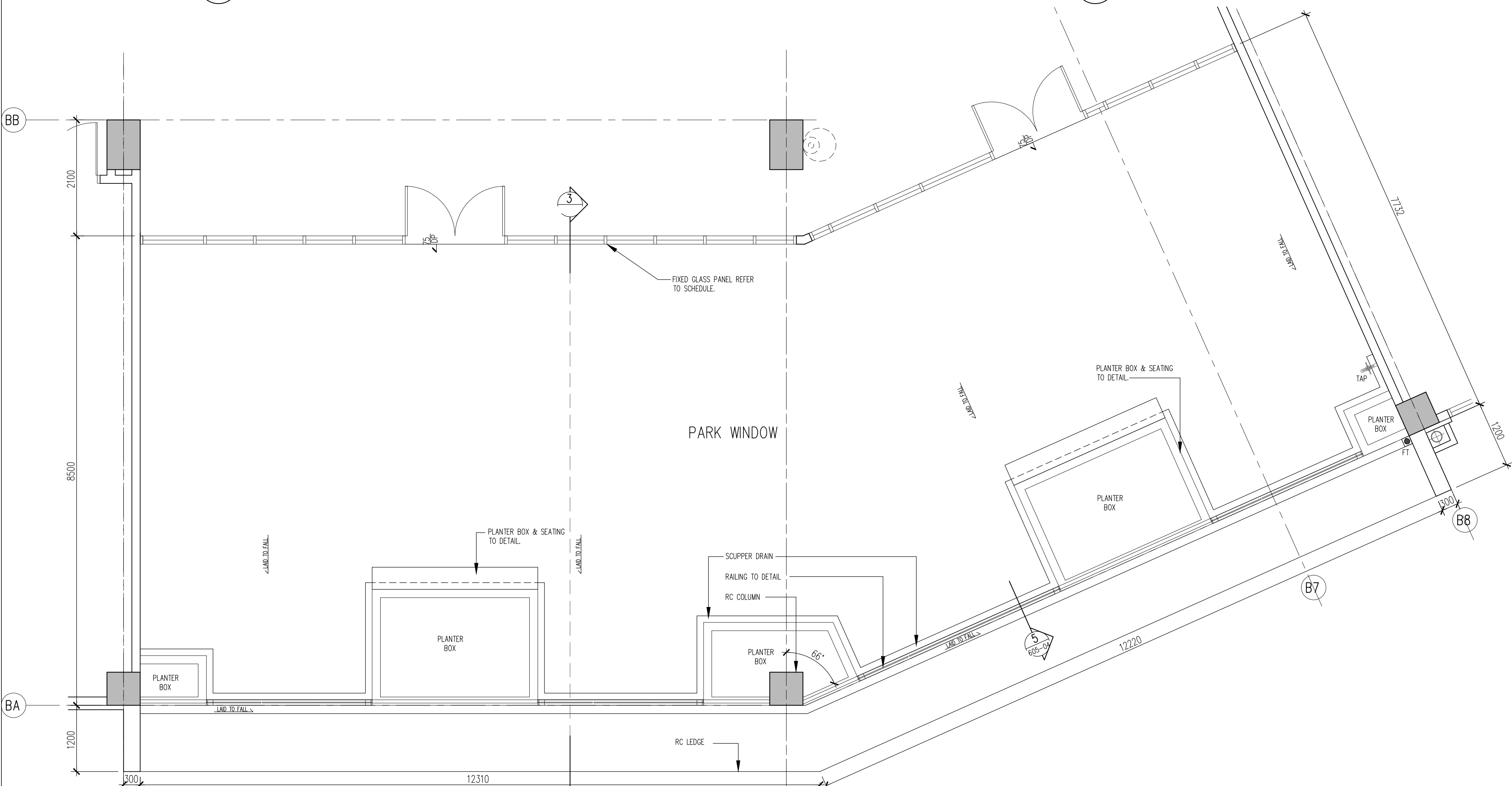
1 PARK WINDOW PLAN - BLOCK B (3RD FLR) SCALE = 1 : 50
