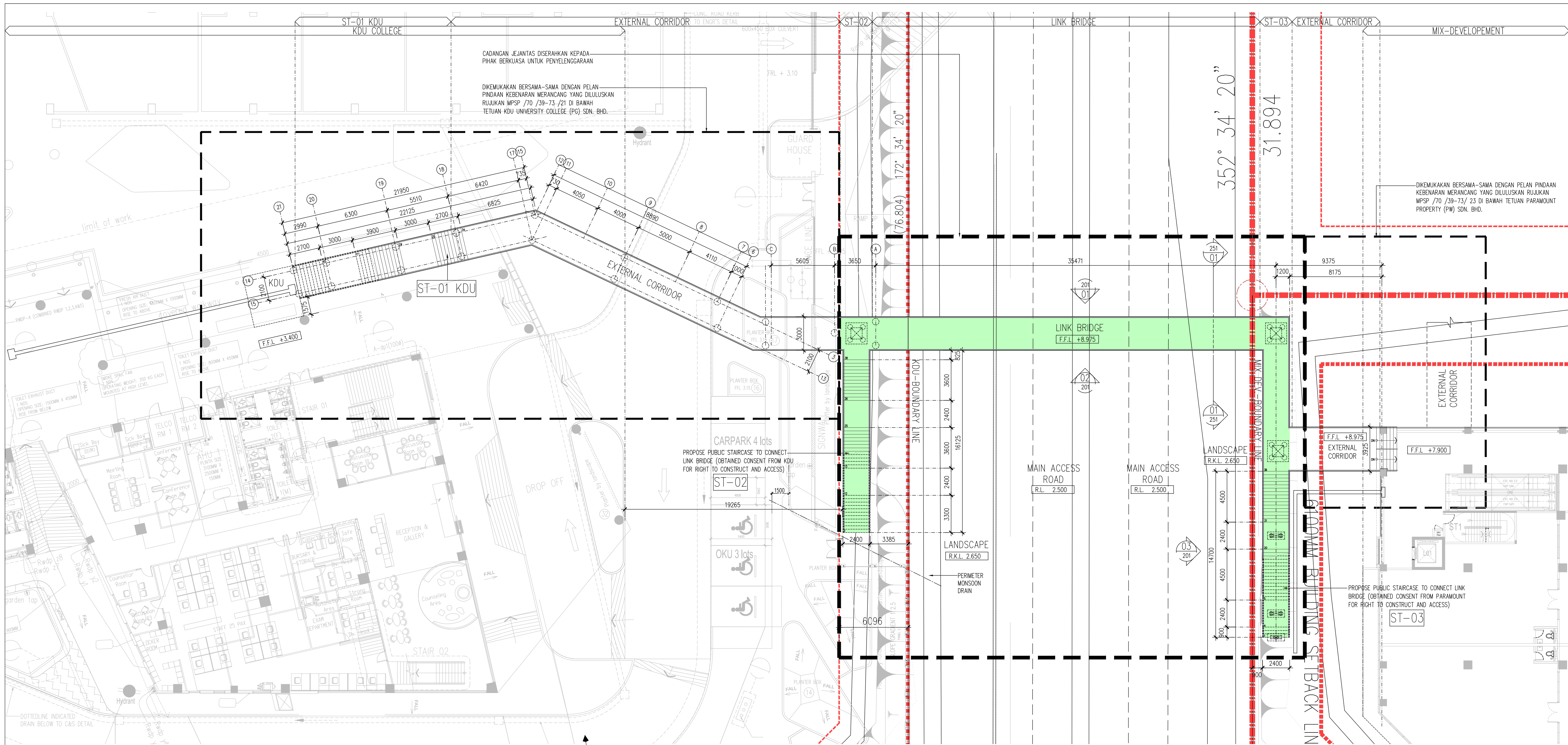
01 PLAN (LINK BRIDGE) SCALE 1:200
