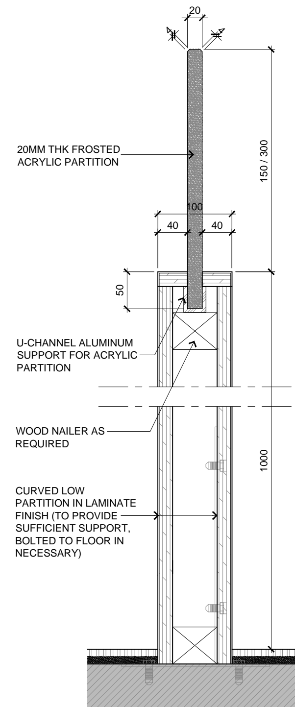
3 TRAINING RESTAURANT 2 SECTION DETAILS SCALE 1:5
