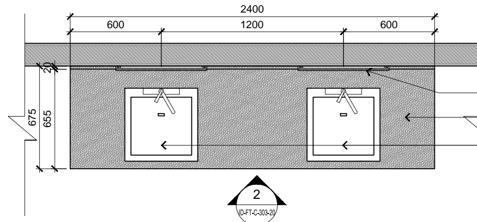
BLOCK C 1ST FLOOR - HOSPITALITY SUITE TOILET LAVATORY PLAN
