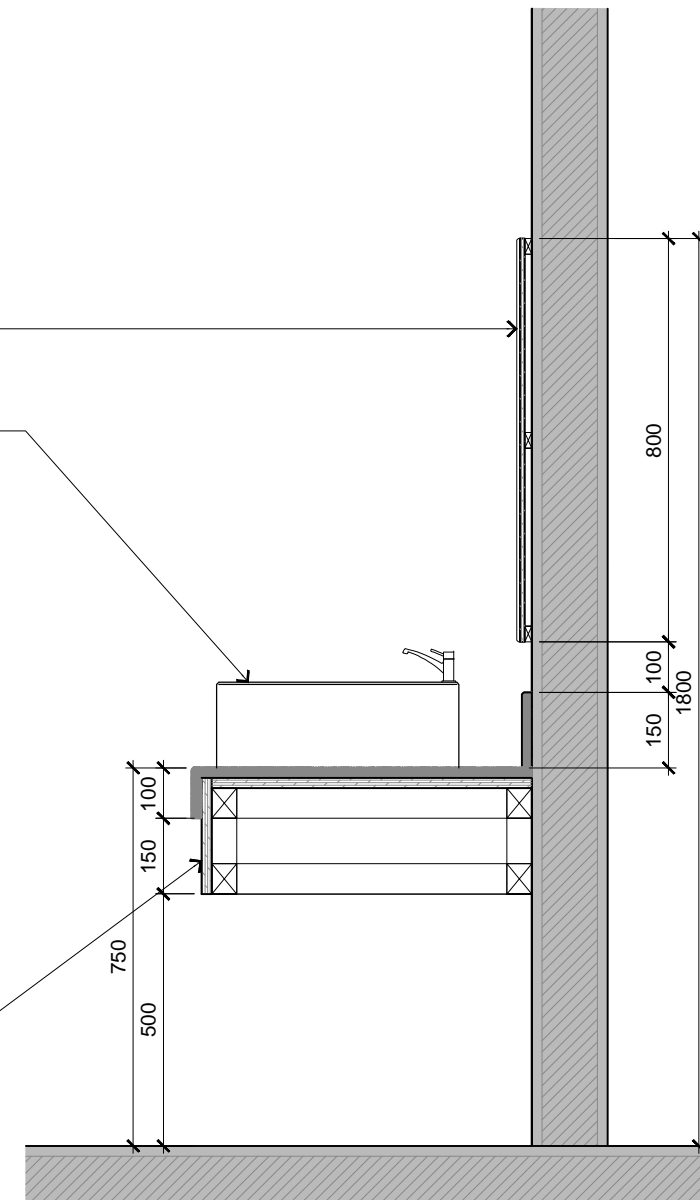
BLOCK C 1ST FLOOR - HOSPITALITY SUITE TOILET LAVATORY SECTION DETAIL
