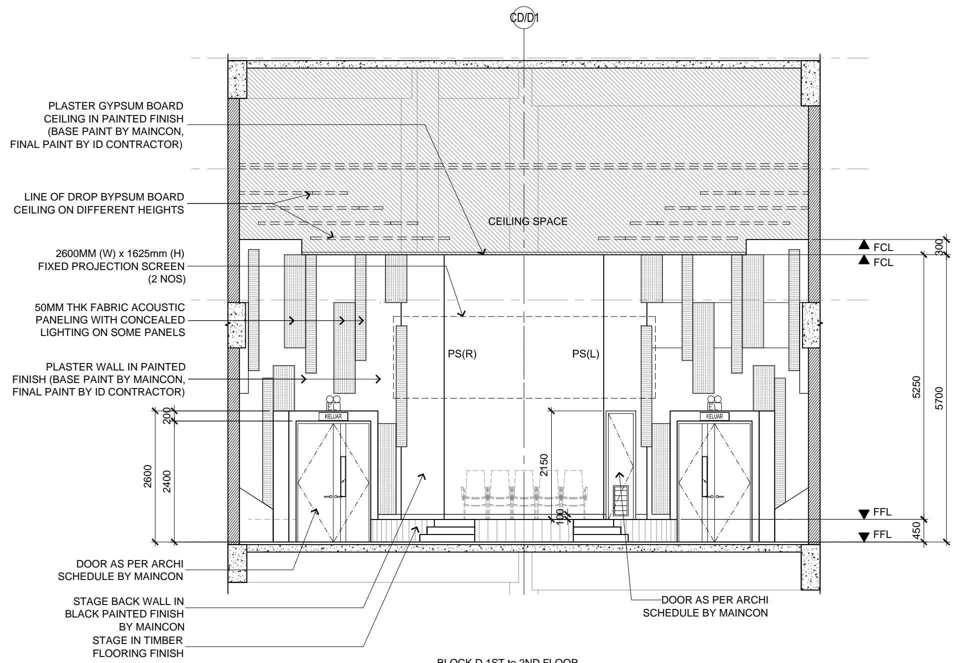
3 BLOCK D 1ST to 2ND FLOOR LECTURE THEATRE ELEVATION 3 SCALE 1:75
