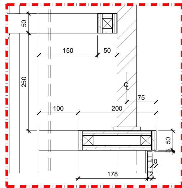
DETAIL A
