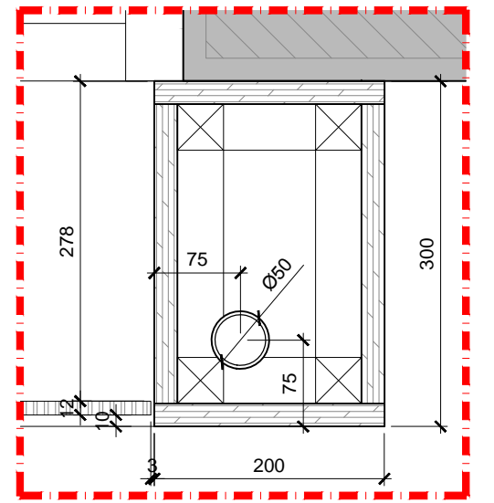
DETAIL D
