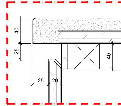
DETAIL E
