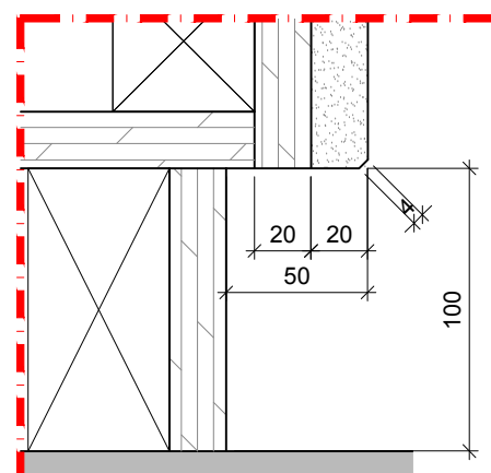
DETAIL D
