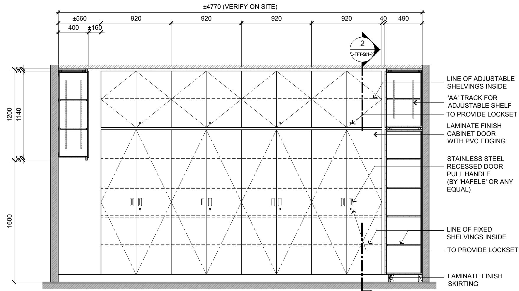
11 BLOCK A 3RD & 4TH FLOOR - OFFICE AUTOMATION FULL HEIGHT CABINET ELEVATION SCALE 1:30
