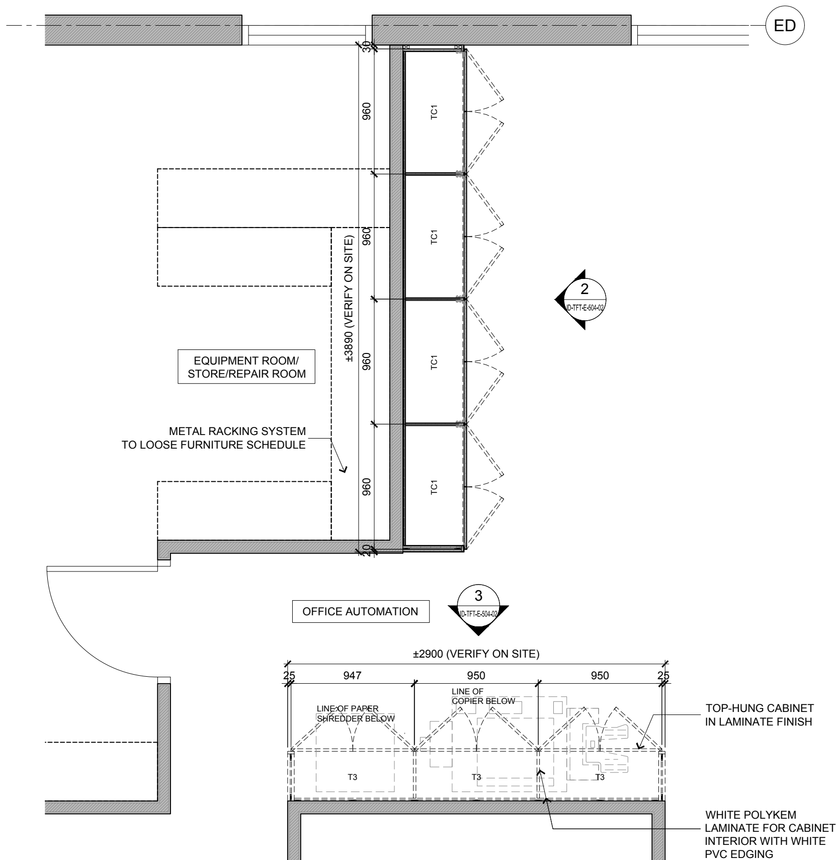
1 BLOCK E 2ND FLR - INFORMATION MANAGEMENT CENTER FULL HEIGHT & TOP HUNG CABINET PLAN SCALE 1:30
