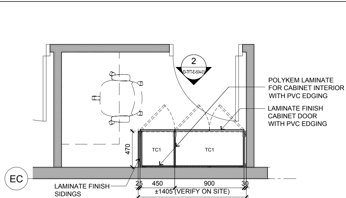
BLOCK E 3RD FLR - PODCAST/FILM STUDIO STORE ROOM FULL HEIGHT CABINET PLAN
