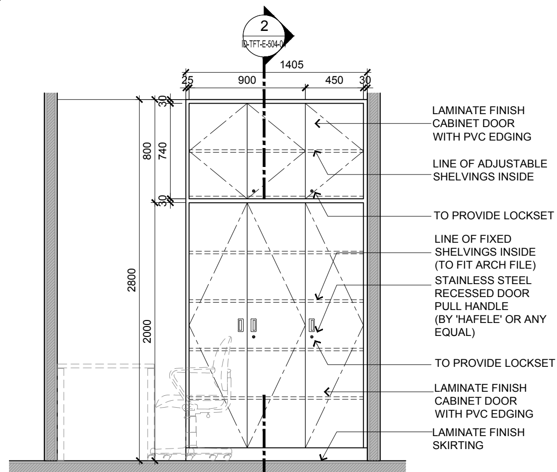
BLOCK E 3RD FLR - PODCAST/FILM STUDIO STORE ROOM FULL HEIGHT CABINET ELEVATION
