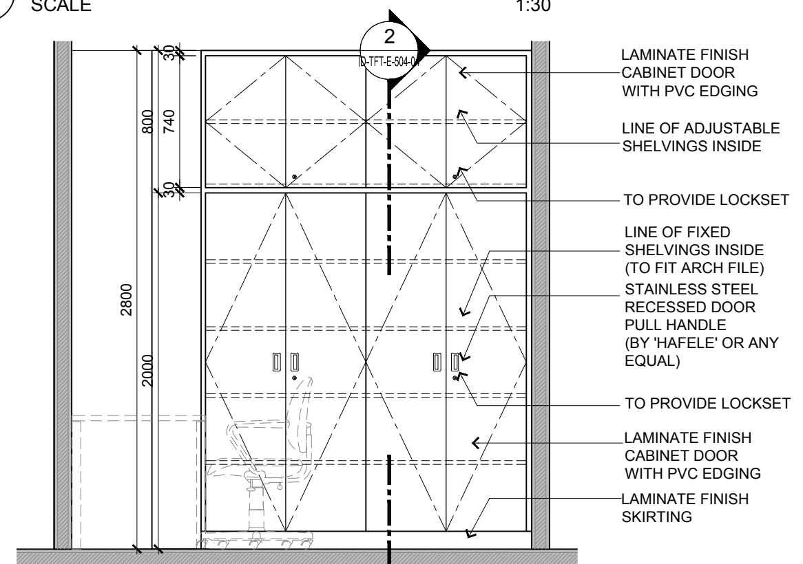
BLOCK E 3RD FLR - ACOUSTIC RADIO STORE ROOM FULL HEIGHT CABINET ELEVATION
