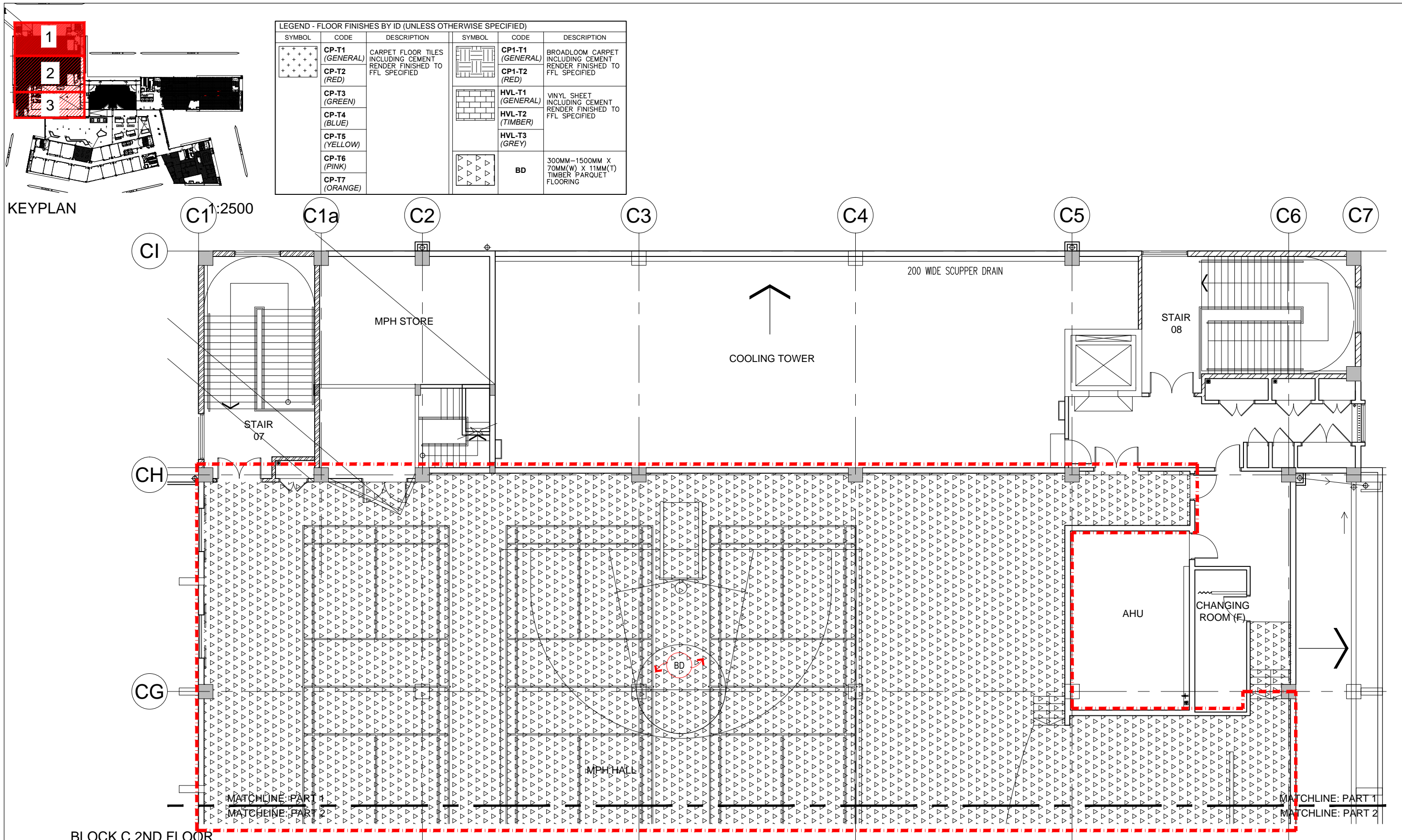
1 BLOCK C 2ND FLOOR FLOOR FINISHES PLAN-PART 1
