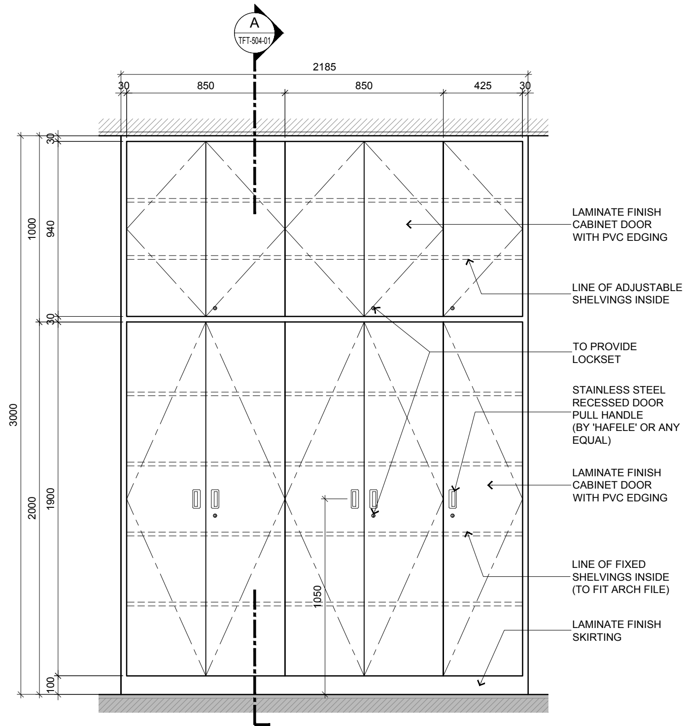
3 BLOCK A 1ST FLOOR - ACADEMIC STAFF DEPT FULL HEIGHT CABINET ELEVATION DETAILS SCALE 1:20
