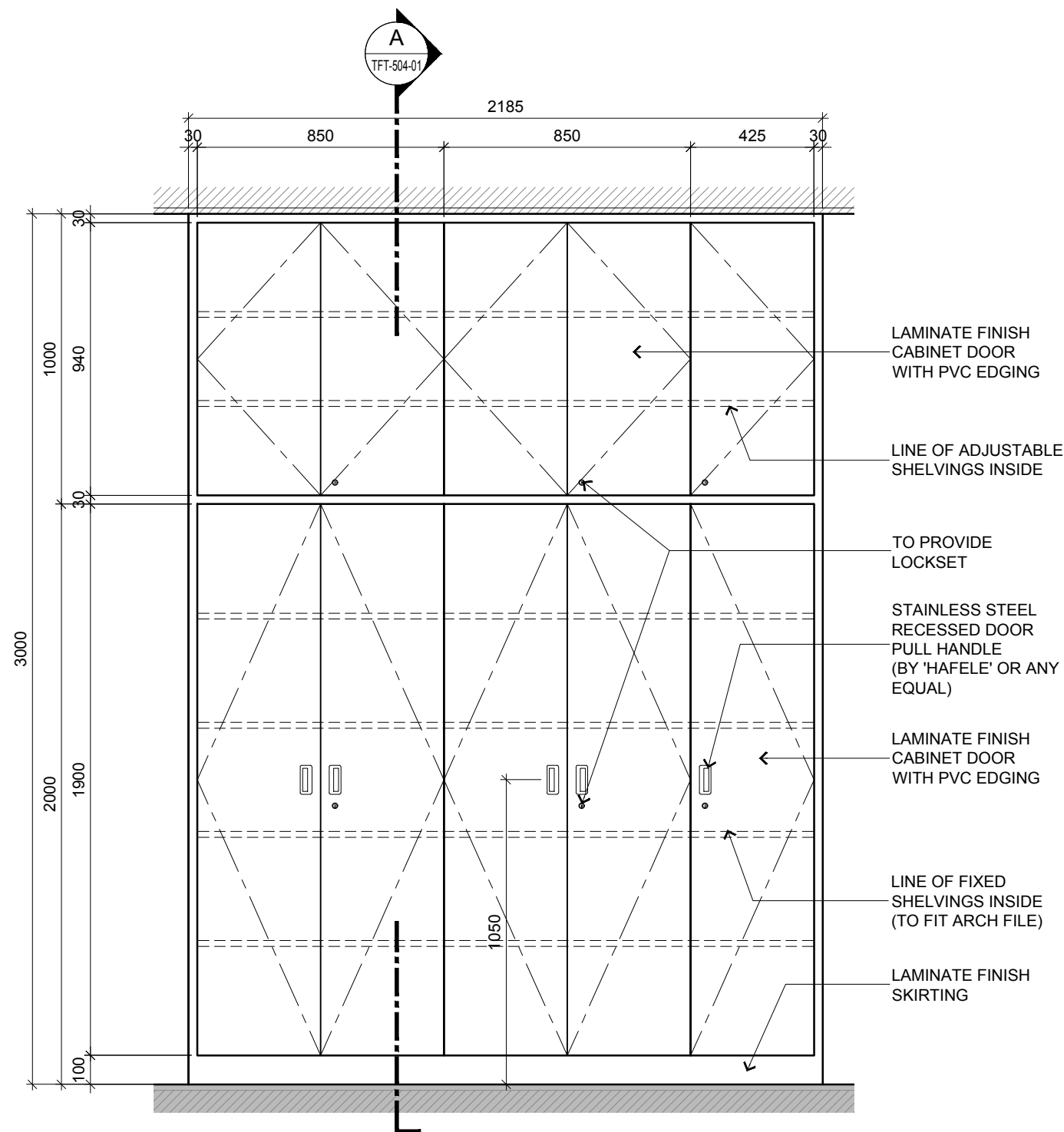
BLOCK A 1ST FLOOR - ACADEMIC STAFF DEPT 3 FULL HEIGHT CABINET ELEVATION DETAILS SCALE 1:20
