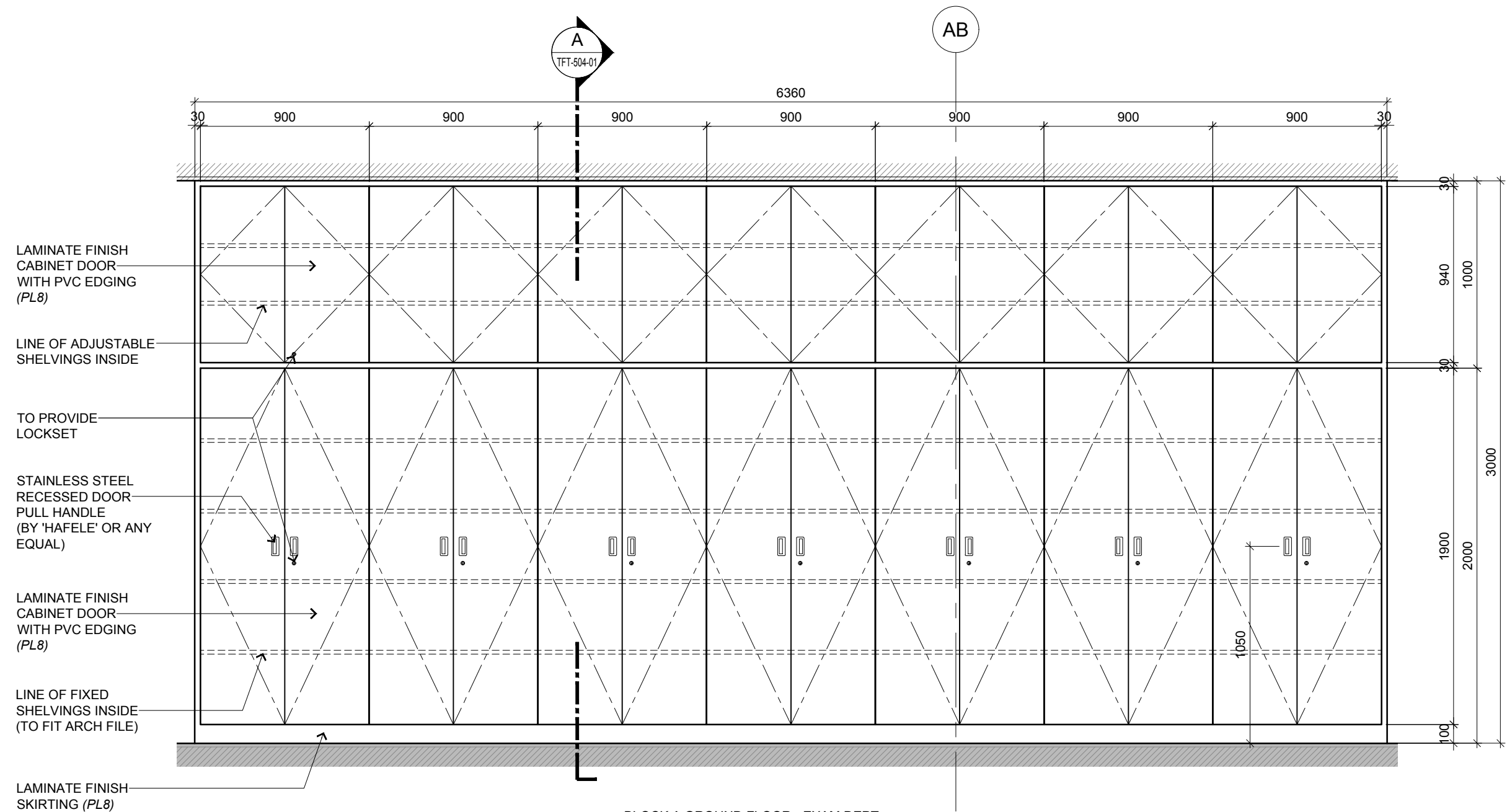
2 BLOCK A GROUND FLOOR - EXAM DEPT FULL HEIGHT CABINET ELEVATION DETAILS SCALE 1:25
