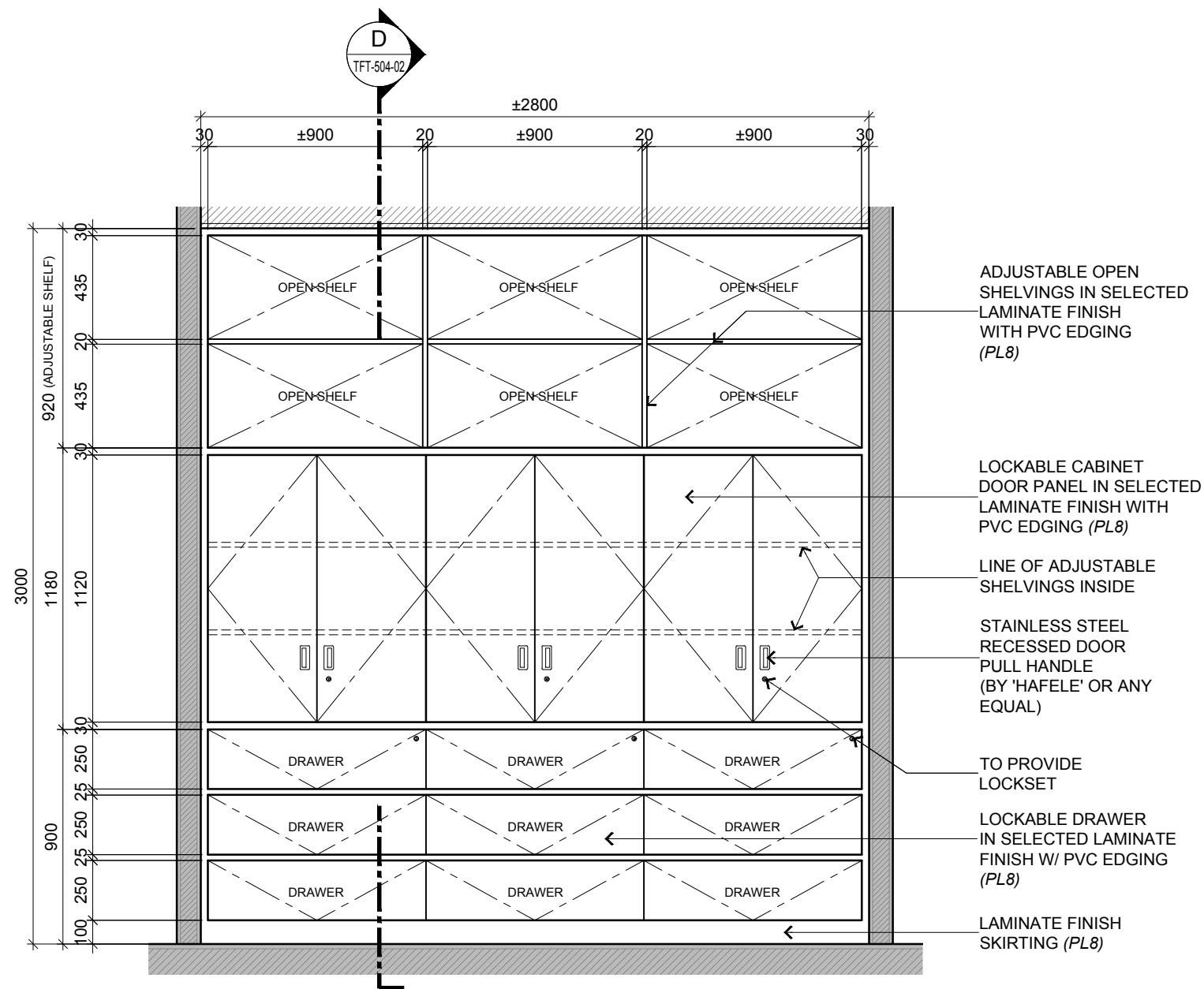
7 BLOCK A GROUND FLOOR - STRONG ROOM TOP HUNG CABINET ELEVATION DETAILS SCALE 1:25
