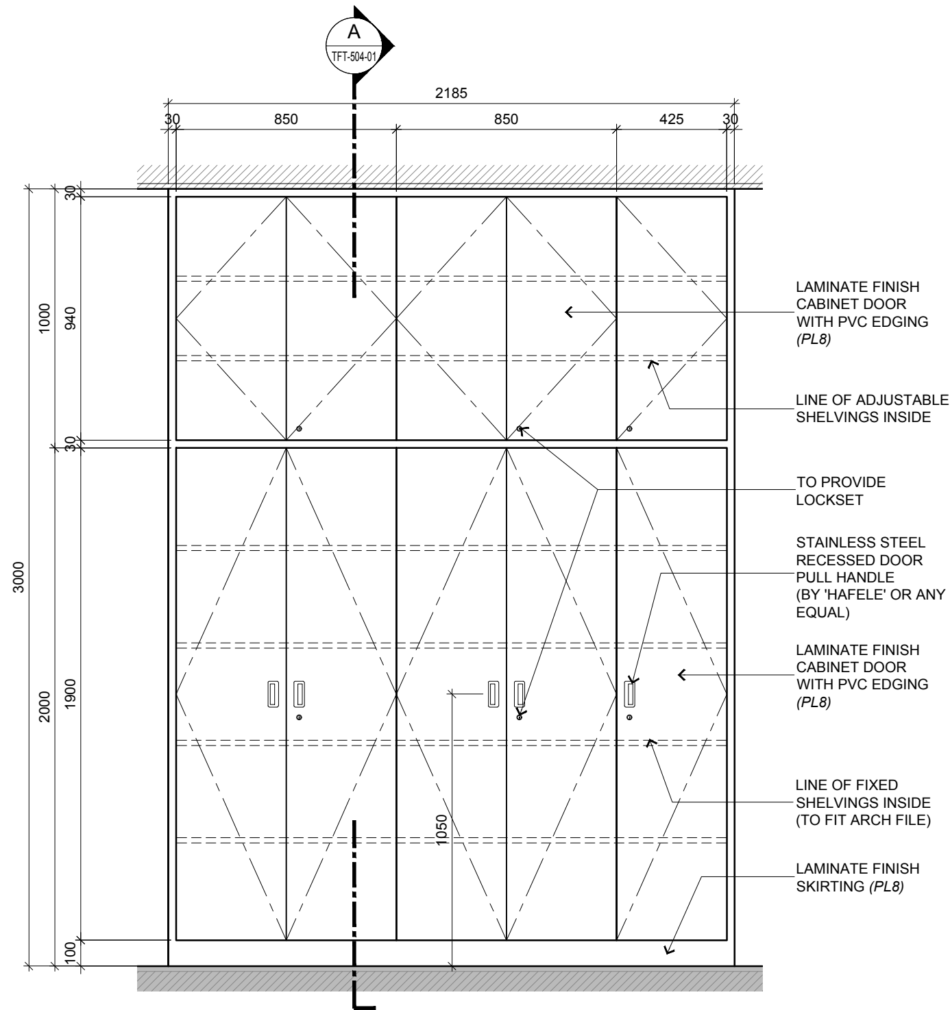
BLOCK A 1ST FLOOR - ACADEMIC STAFF DEPT FULL HEIGHT CABINET ELEVATION DETAILS
