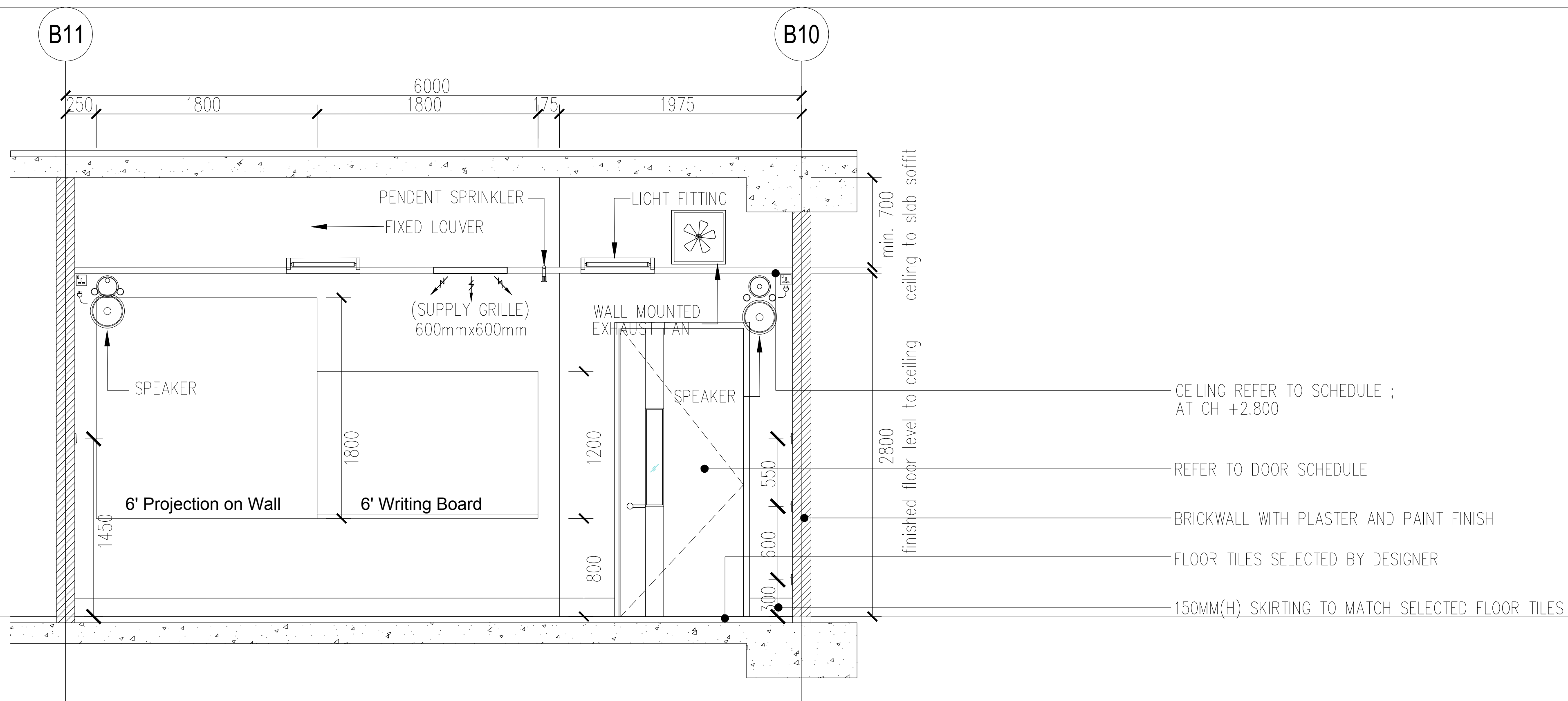
SECTIONAL ELEVATION 1
