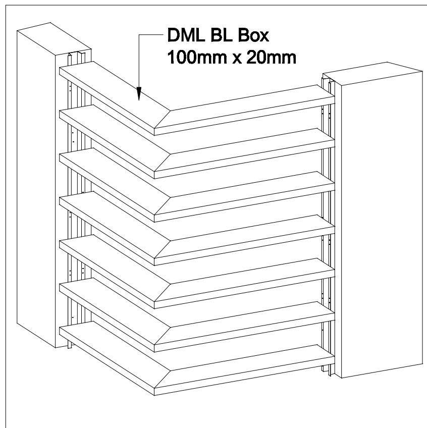
TYPICAL ISOMETRIC VIEW Scale : NTS
