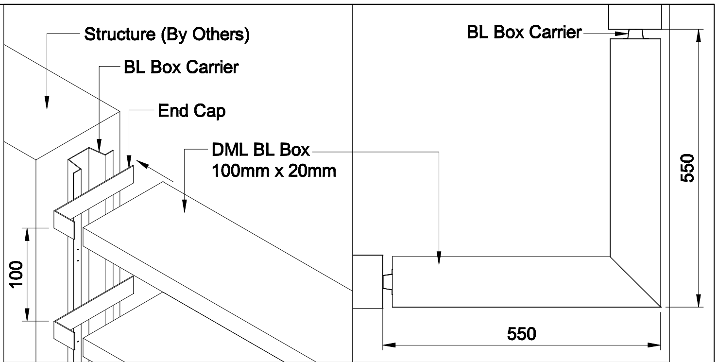
TYPICAL 3D DETAIL Scale : NTS
