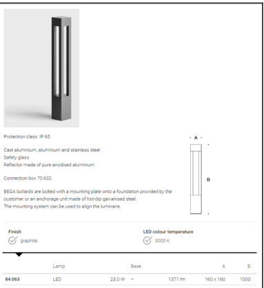
BOLLARD LIGHT
