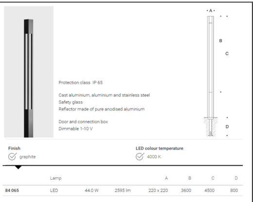
POLE LIGHT
