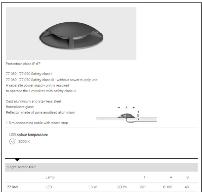
IN-GROUND LIGHT
