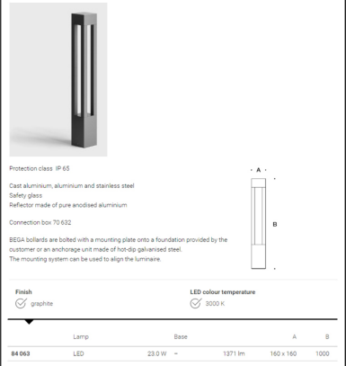
BOLLARD LIGHT
