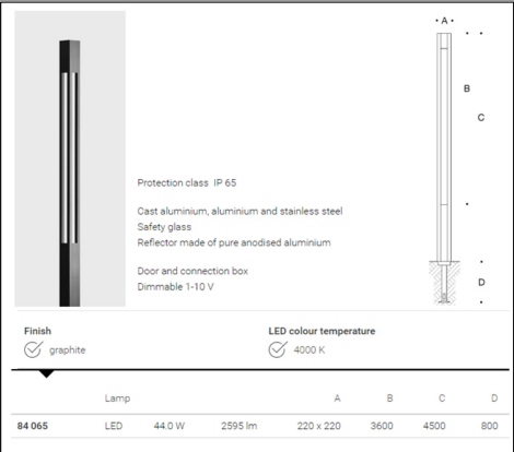
POLE LIGHT
