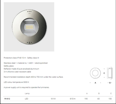
UNDERWATER LIGHT
