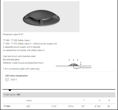
IN-GROUND LIGHT
