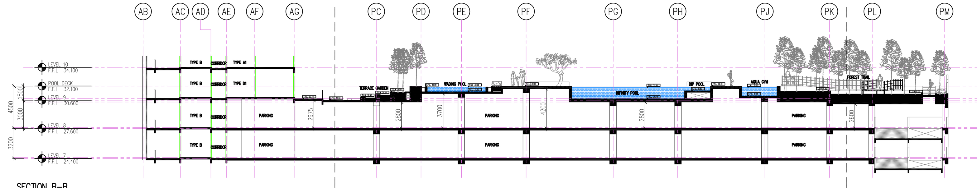
SECTION B-B
