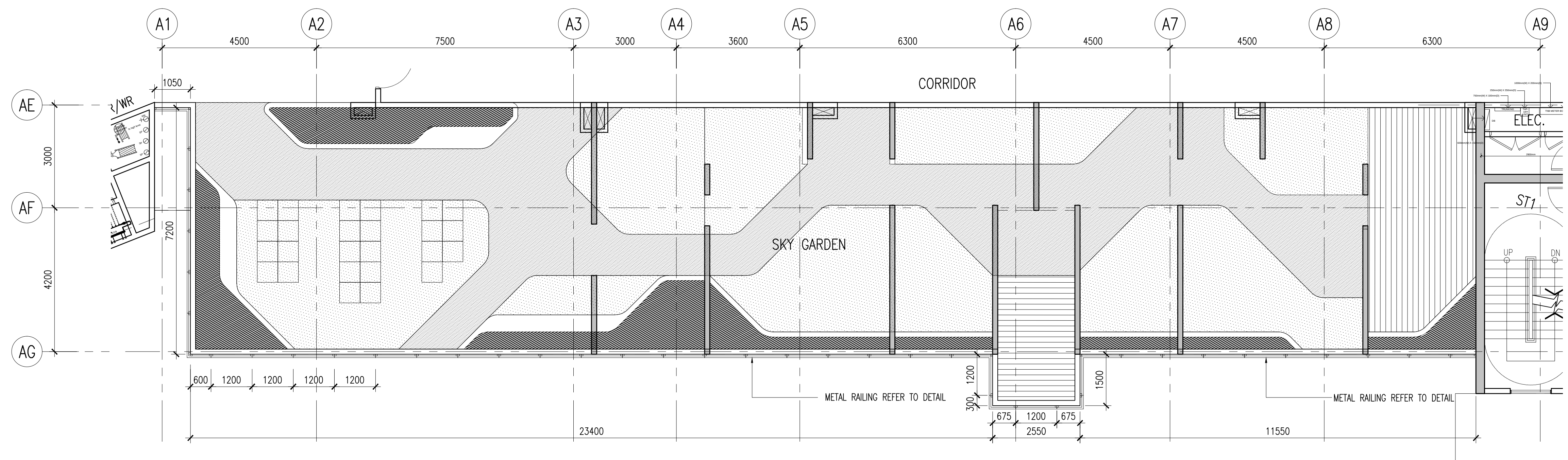
01 LEVEL 120 - SKY GARDEN 567-01 SCALE = 1 : 75
