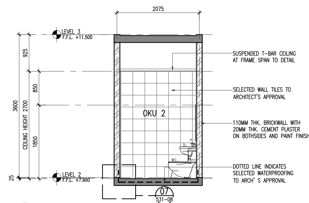
04 TYPICAL SECTION 531-06 SCALE = 1 : 50
