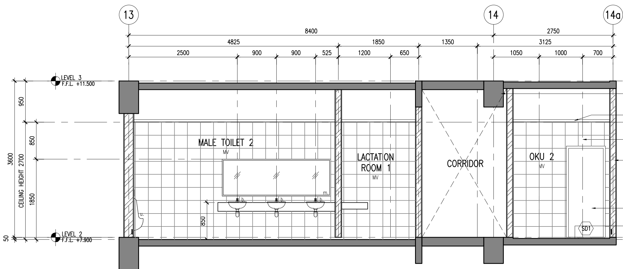
01 TYPICAL SECTION 531-06 SCALE = 1 : 50
