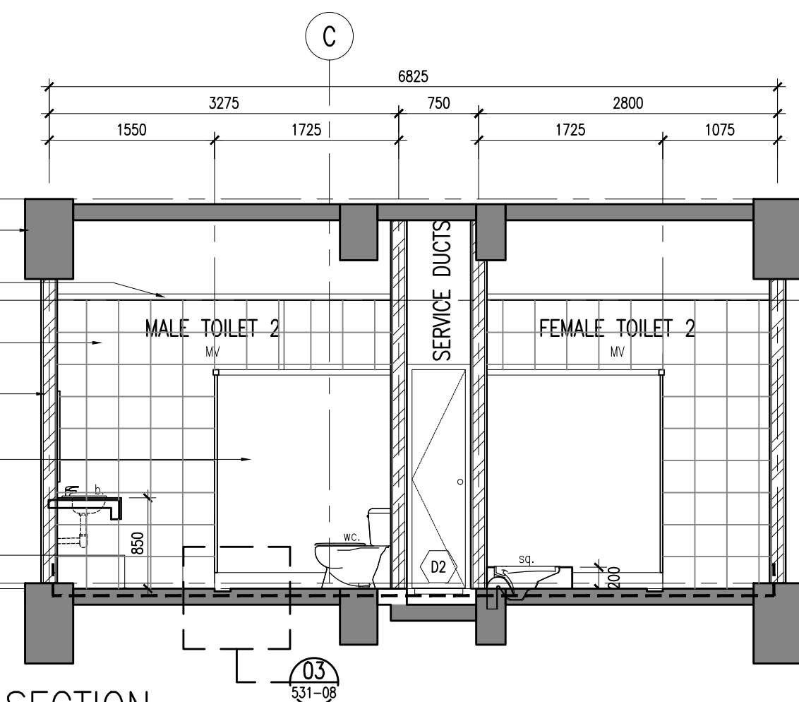
02 TYPICAL SECTION 531-06 SCALE = 1 : 50
