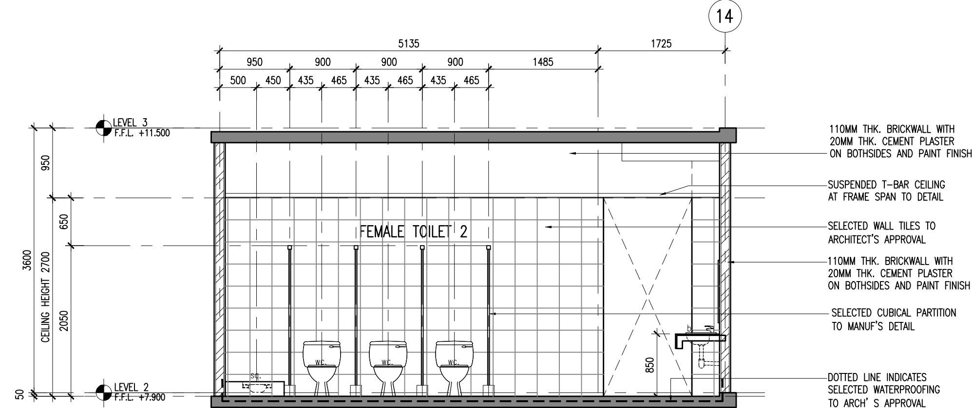
03 TYPICAL SECTION 531-06 SCALE = 1 : 50
