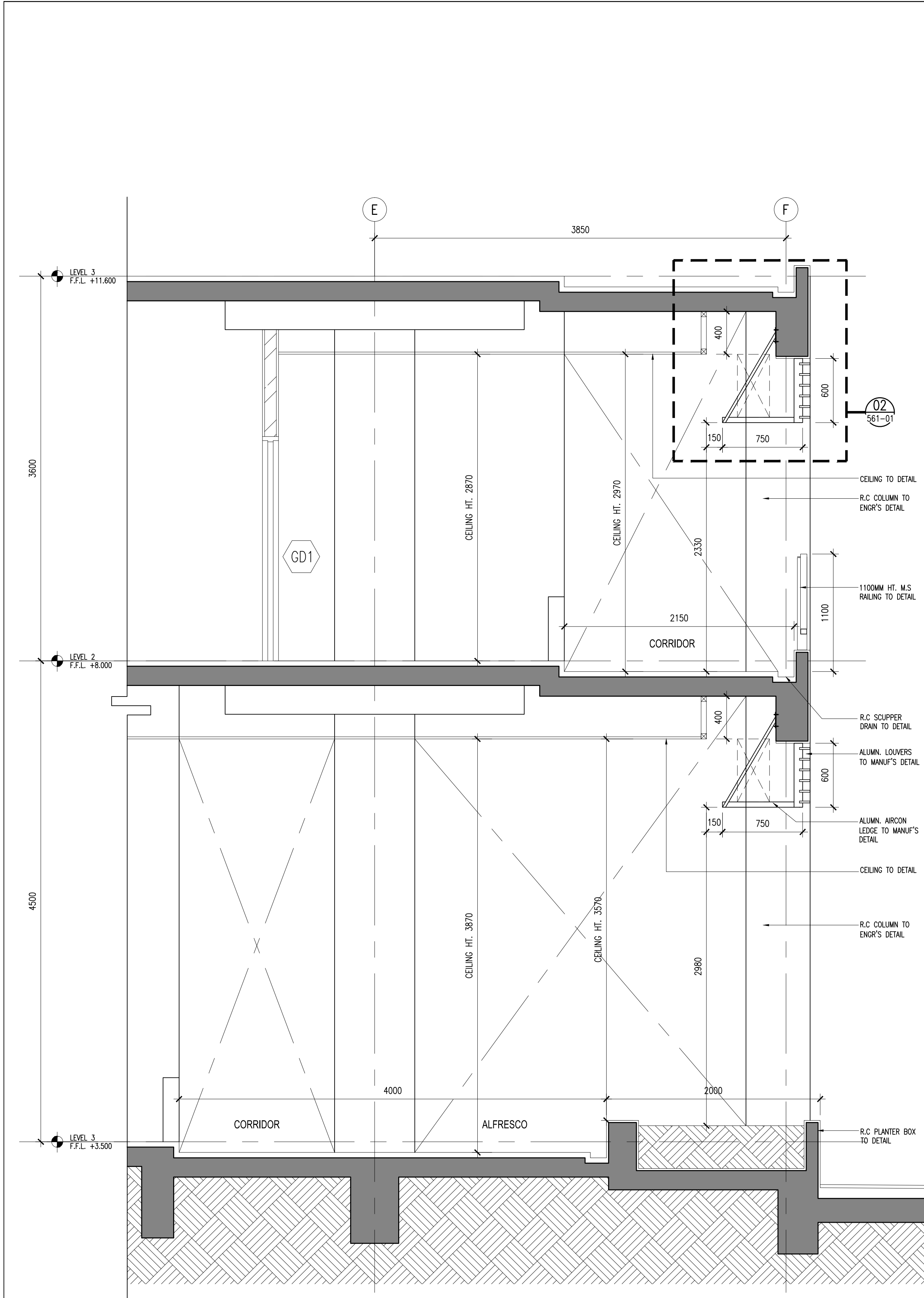
01 LOUVERS DETAIL - SECTION 561-01 SCALE = 1 : 25
