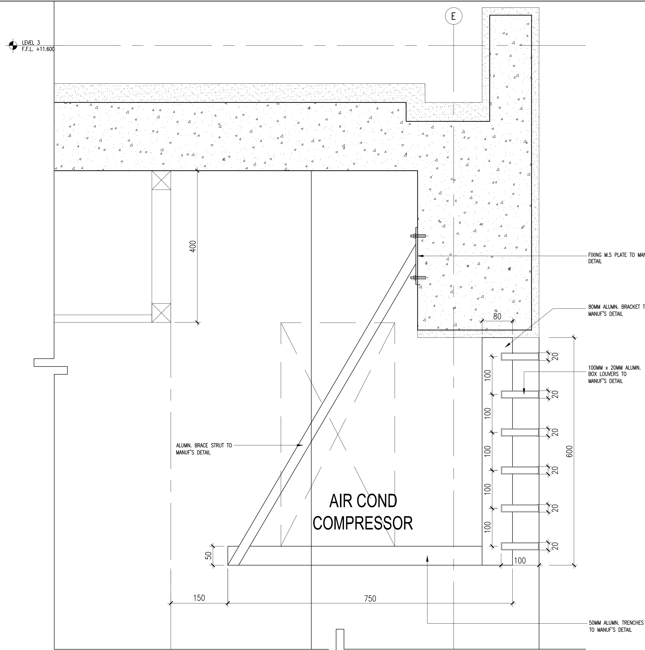
02 LOUVERS DETAIL - BLOW UP 561-01 SCALE = 1 : 5
