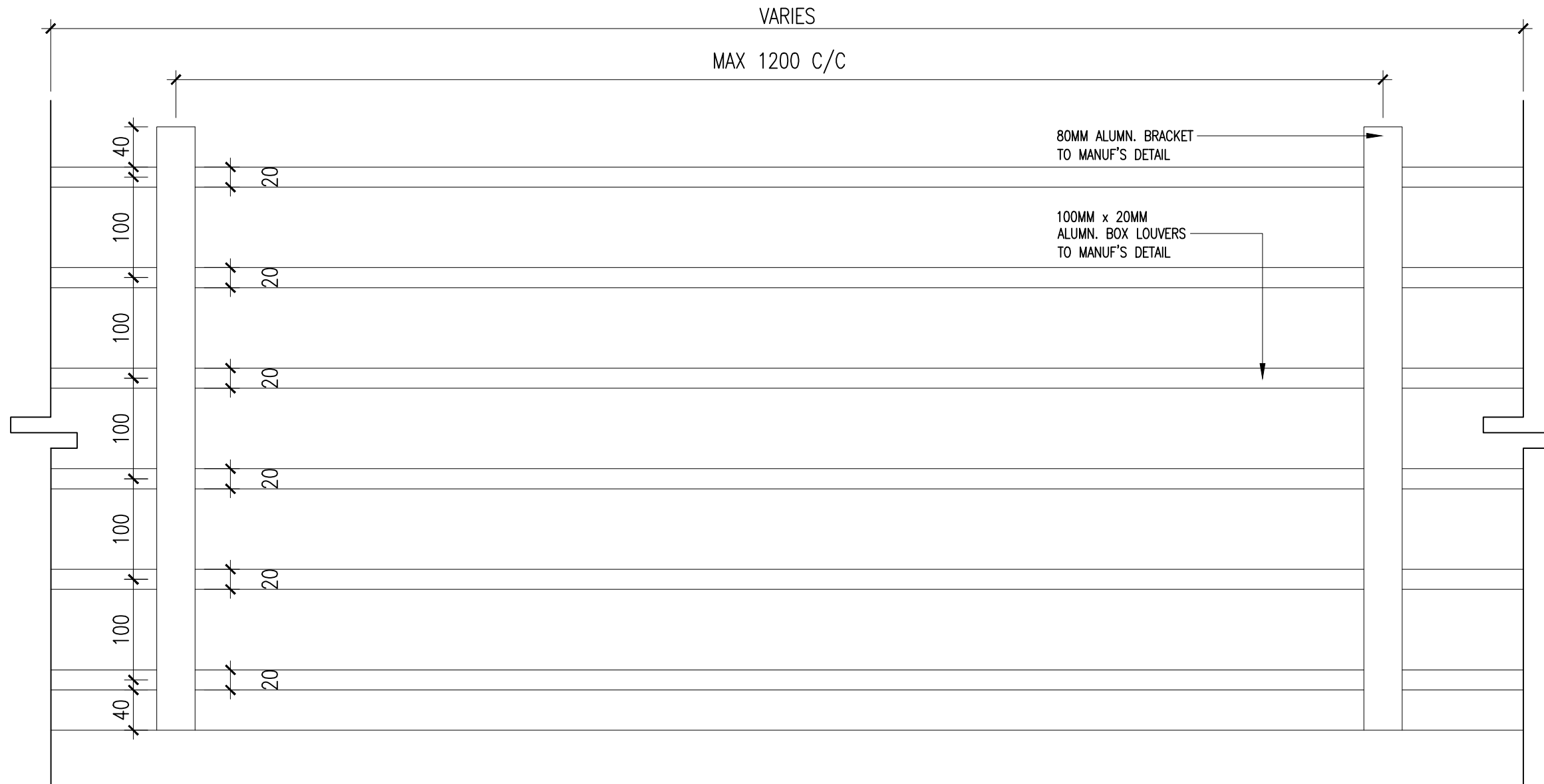
03 LOUVERS DETAIL - FRONT VIEW 561-01 SCALE = 1 : 5
