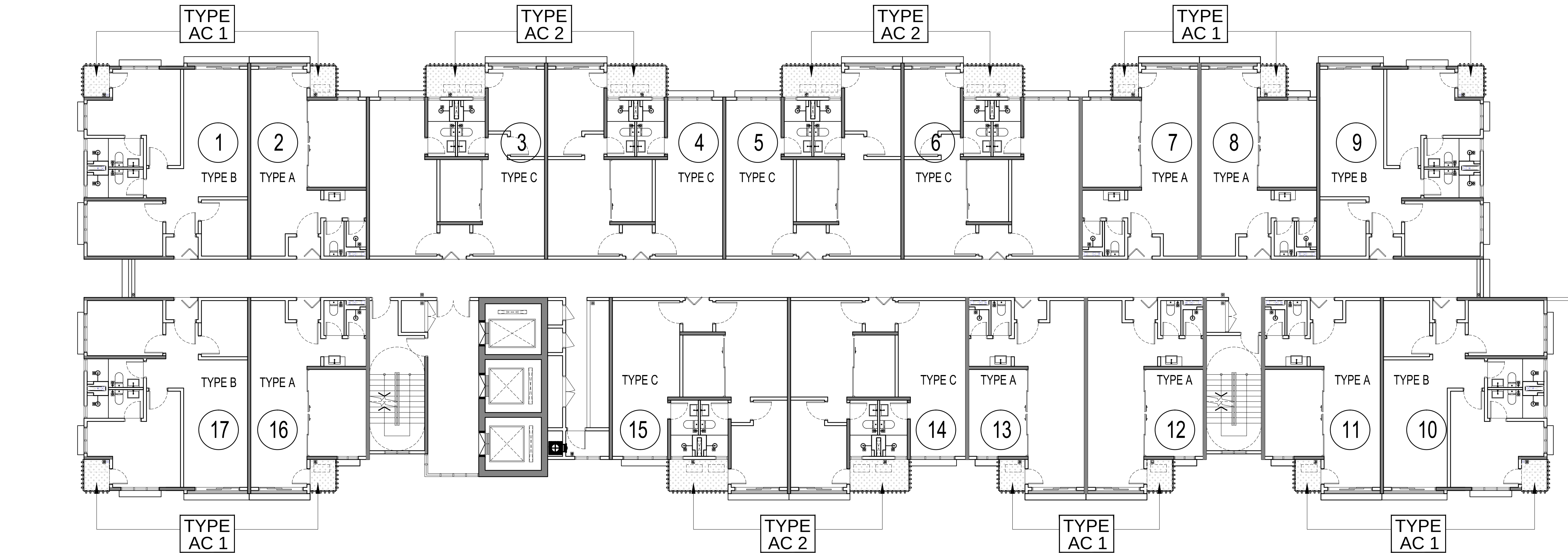
01 AIR-COND LEDGE LOUVERS – LOCATION PLAN BLOCK A 561-04 SCALE = 1 : 100
