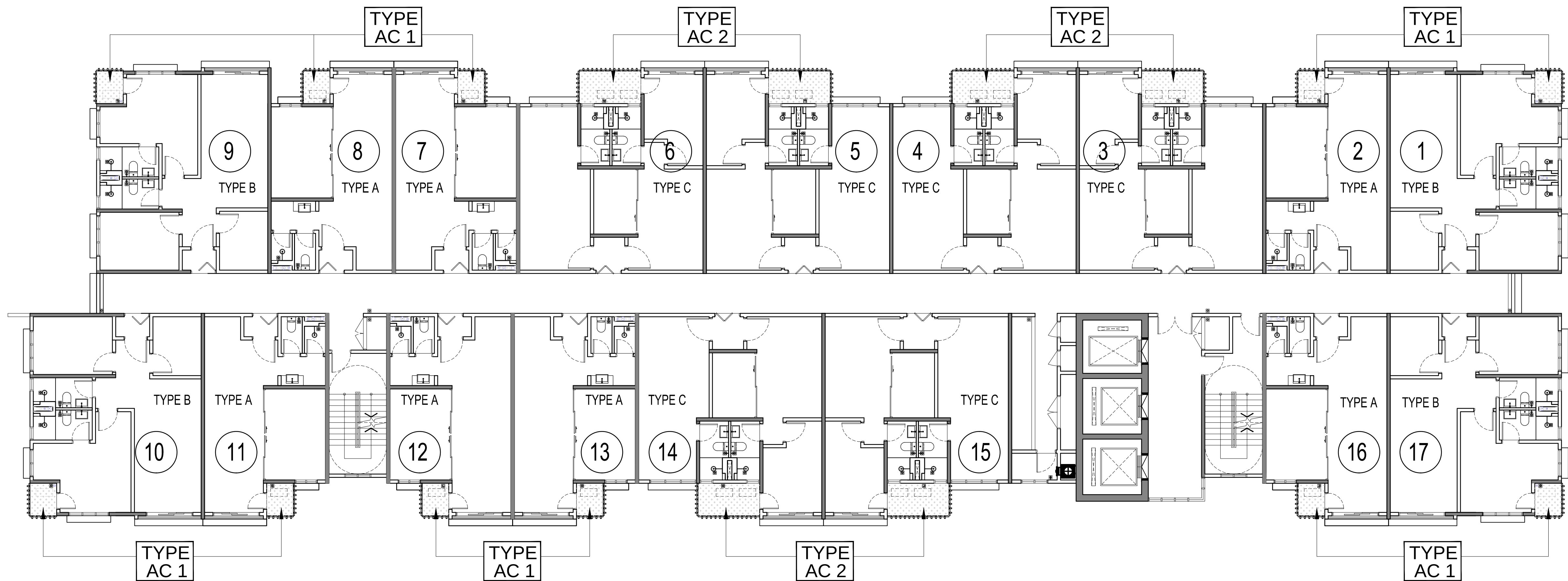
02 AIR-COND LEDGE LOUVERS – LOCATION PLAN BLOCK B 561-04 SCALE = 1 : 100
