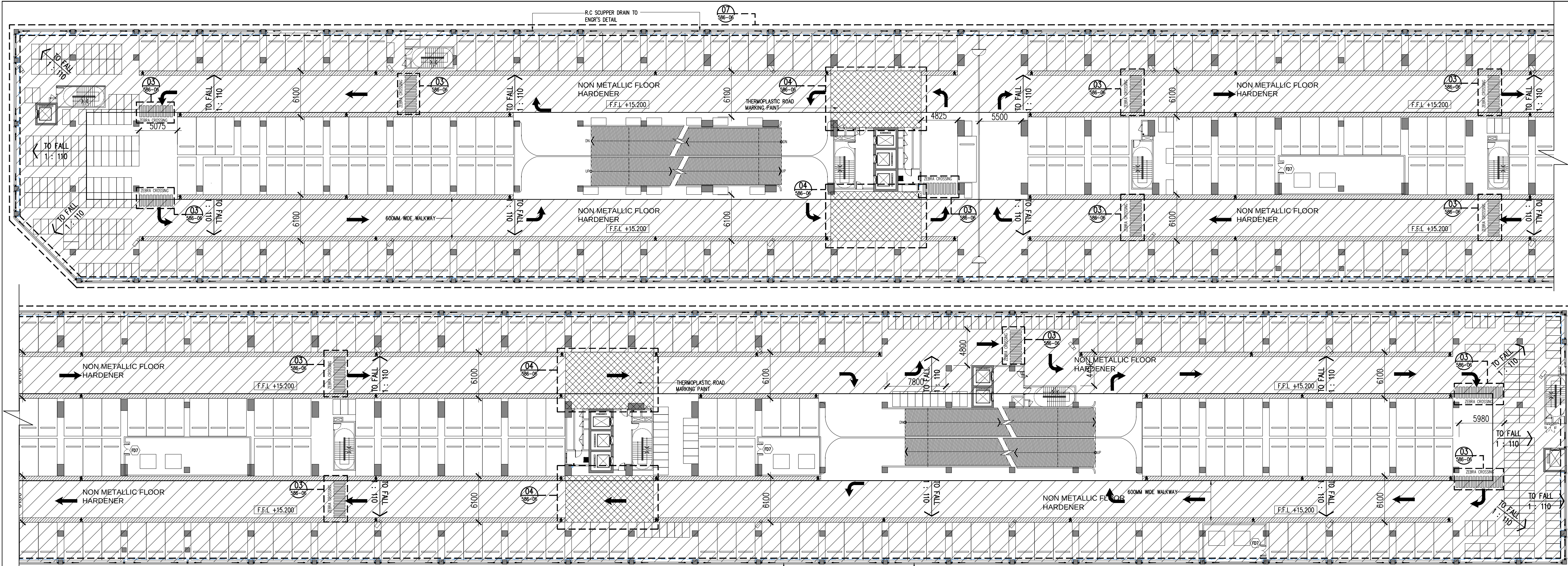
02 CARPARK DETAIL – LEVEL 4
