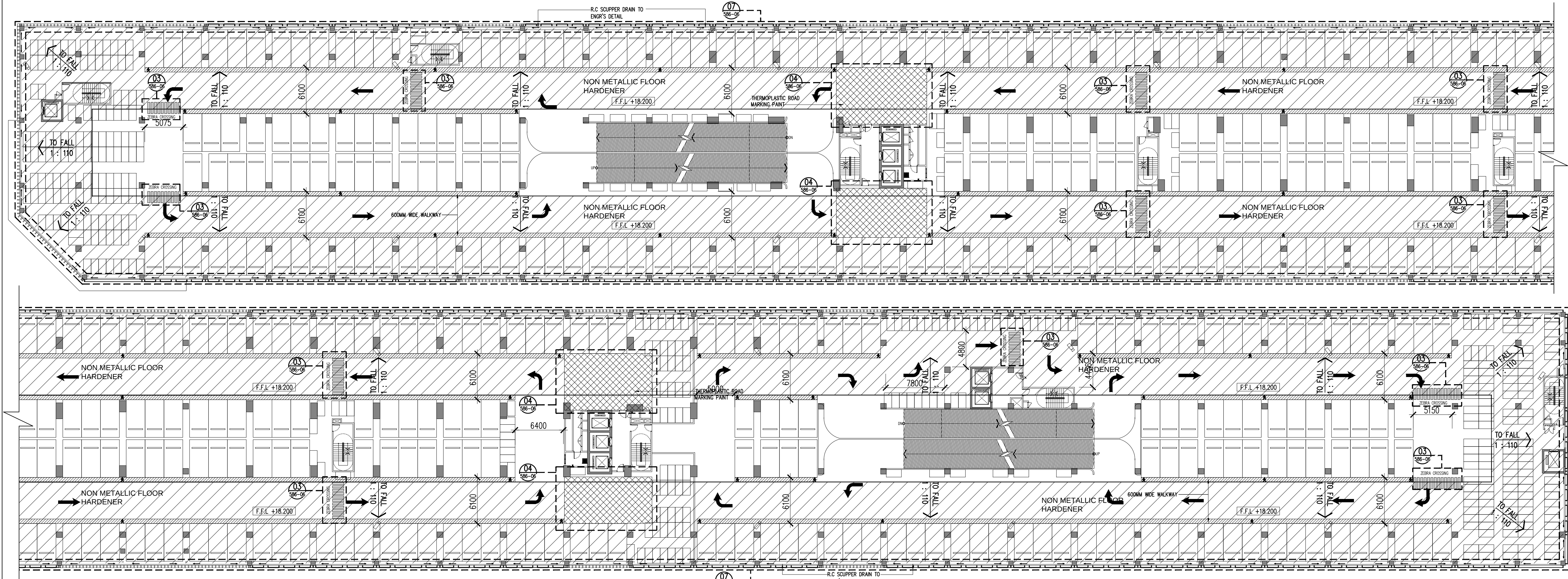
03 CARPARK DETAIL – LEVEL 5&6
