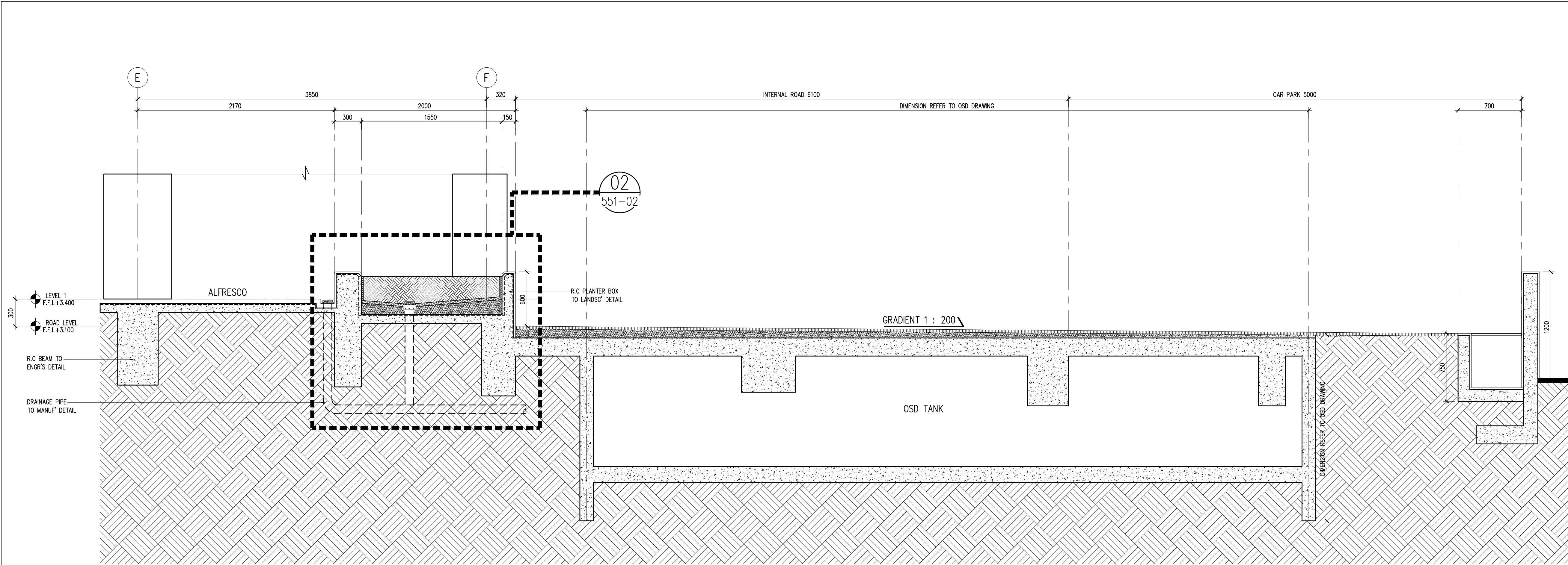
01 TYPICAL SECTION 01 251 SCALE = 1 : 25
