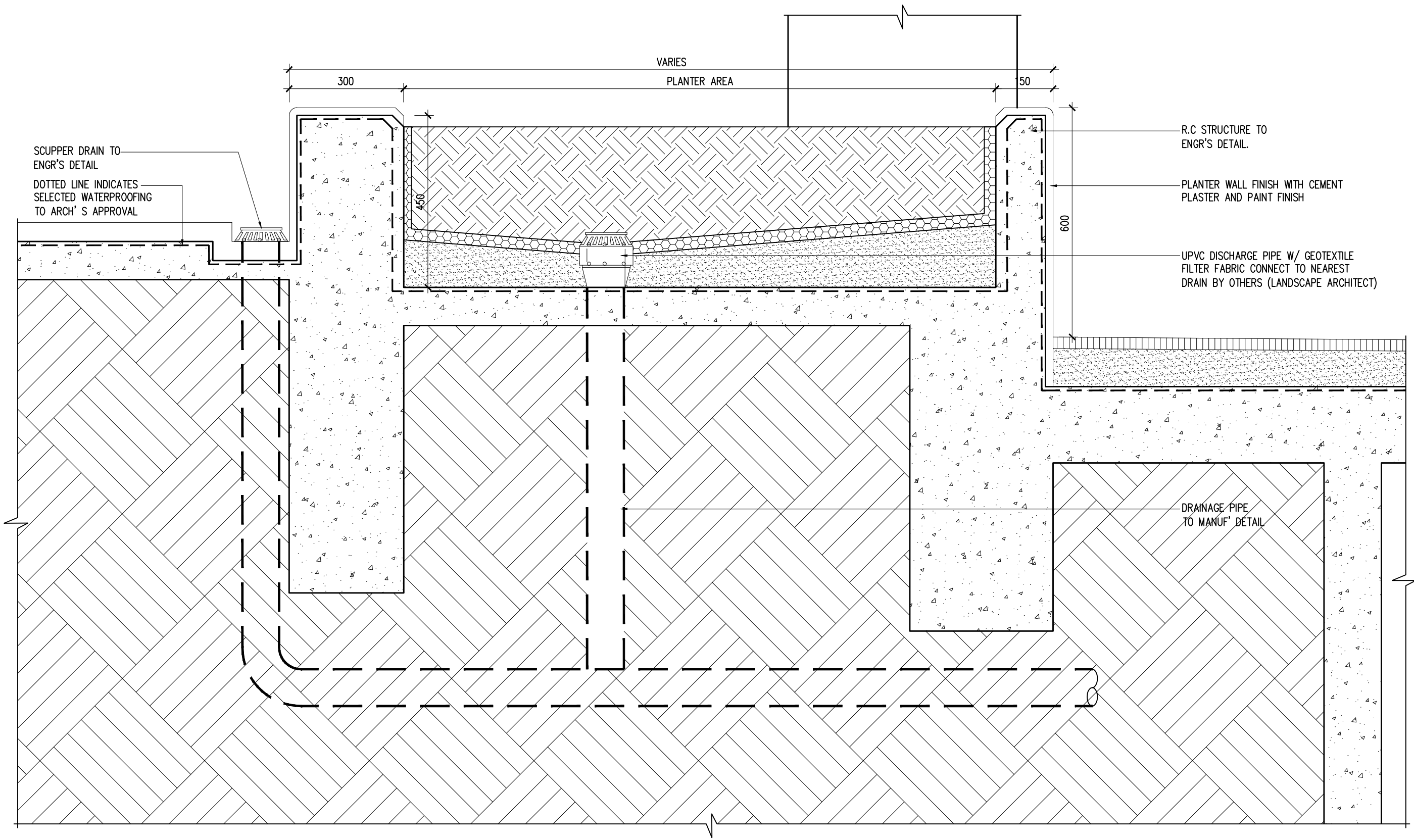
02 TYPICAL DETAIL 251 SCALE = 1 : 5
