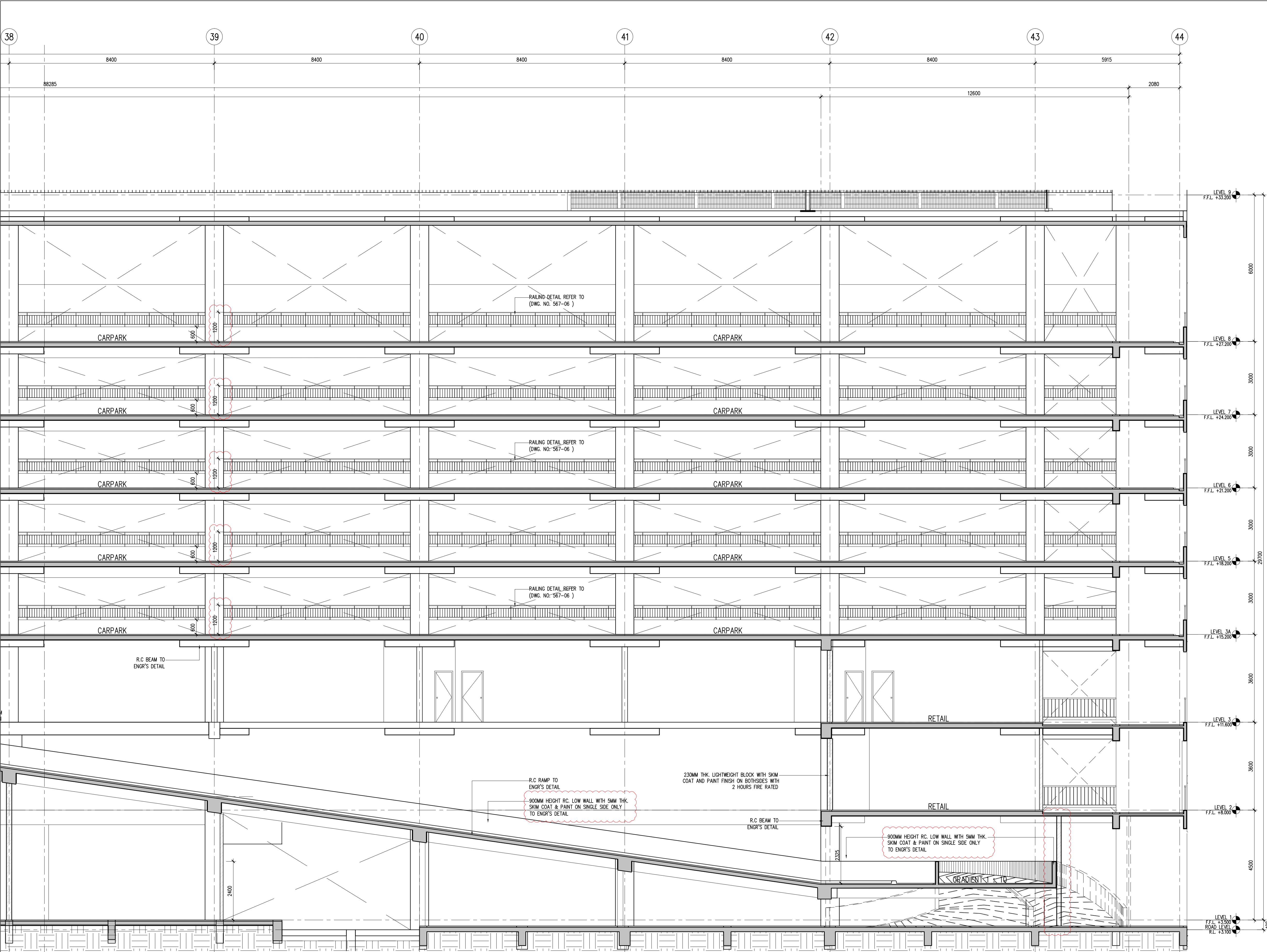
13 SECTION (1 OF 2) 523-09 SCALE = 1 : 75
