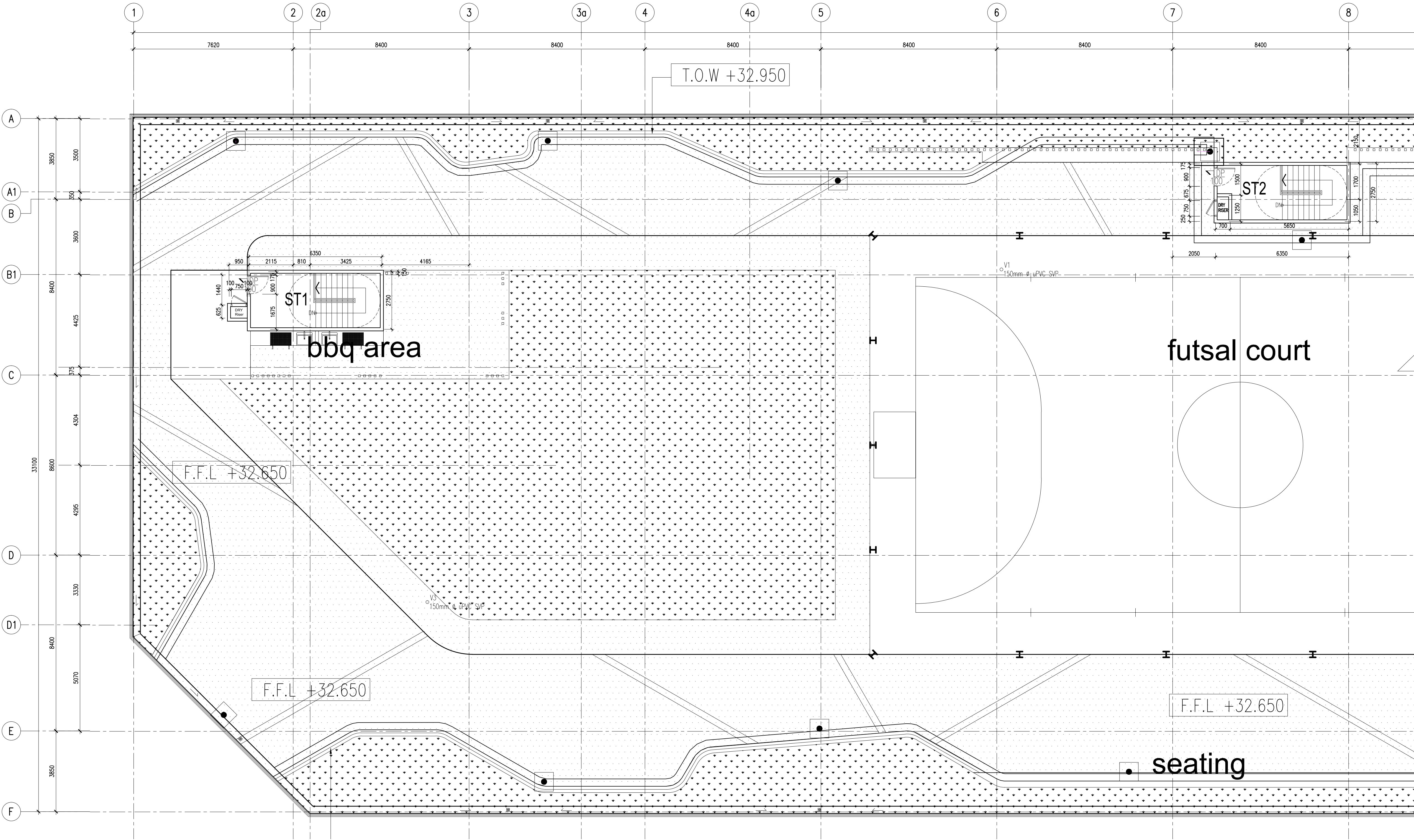
01 BRICKWALL SETTING OUT-LEVEL 9 ( PART 1 OF 7 ) 873-01 SCALE = 1 : 100
