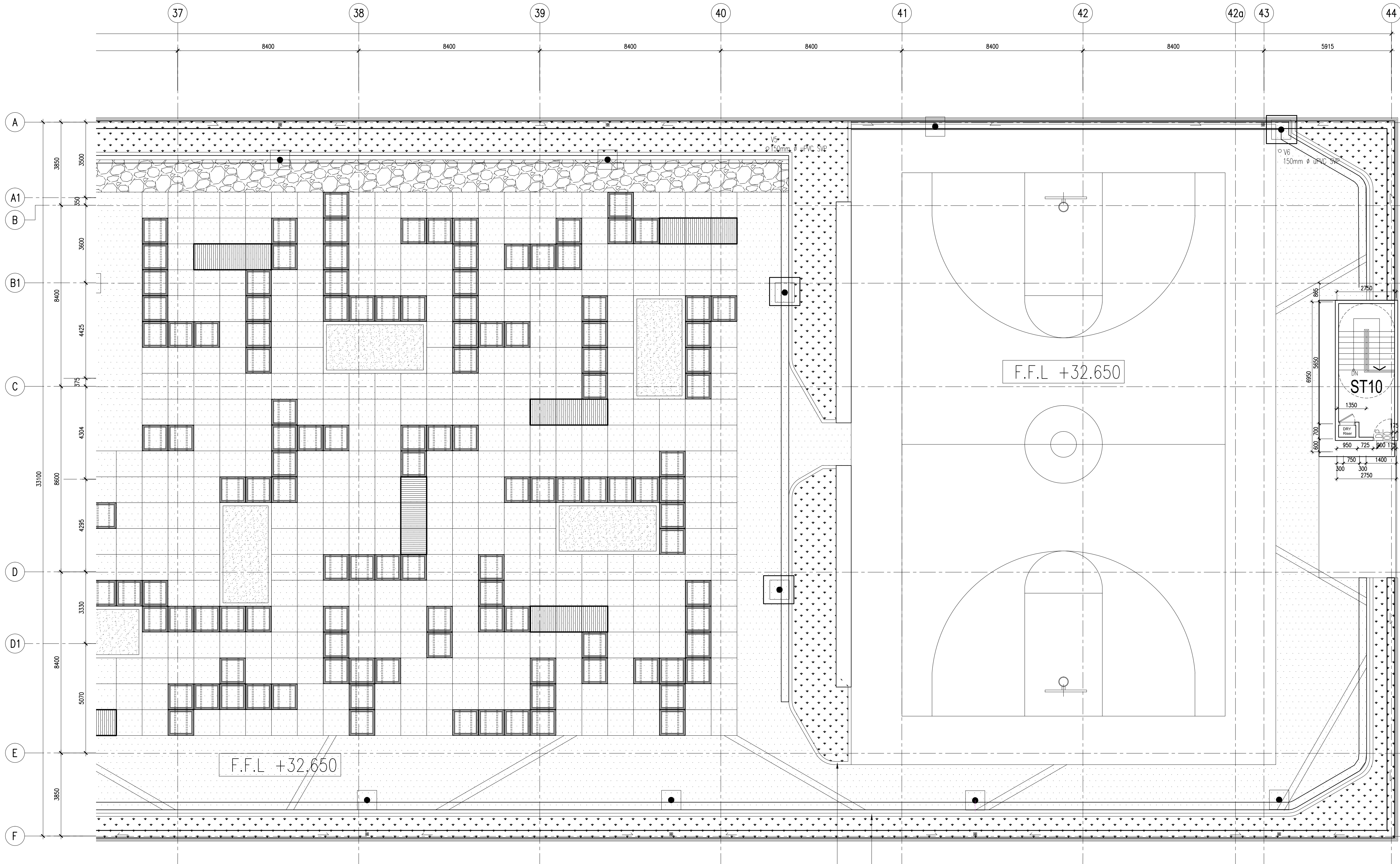
01 BRICKWALL SETTING OUT-LEVEL 9 (PART 7 OF 7) 873-07 SCALE = 1 : 100
