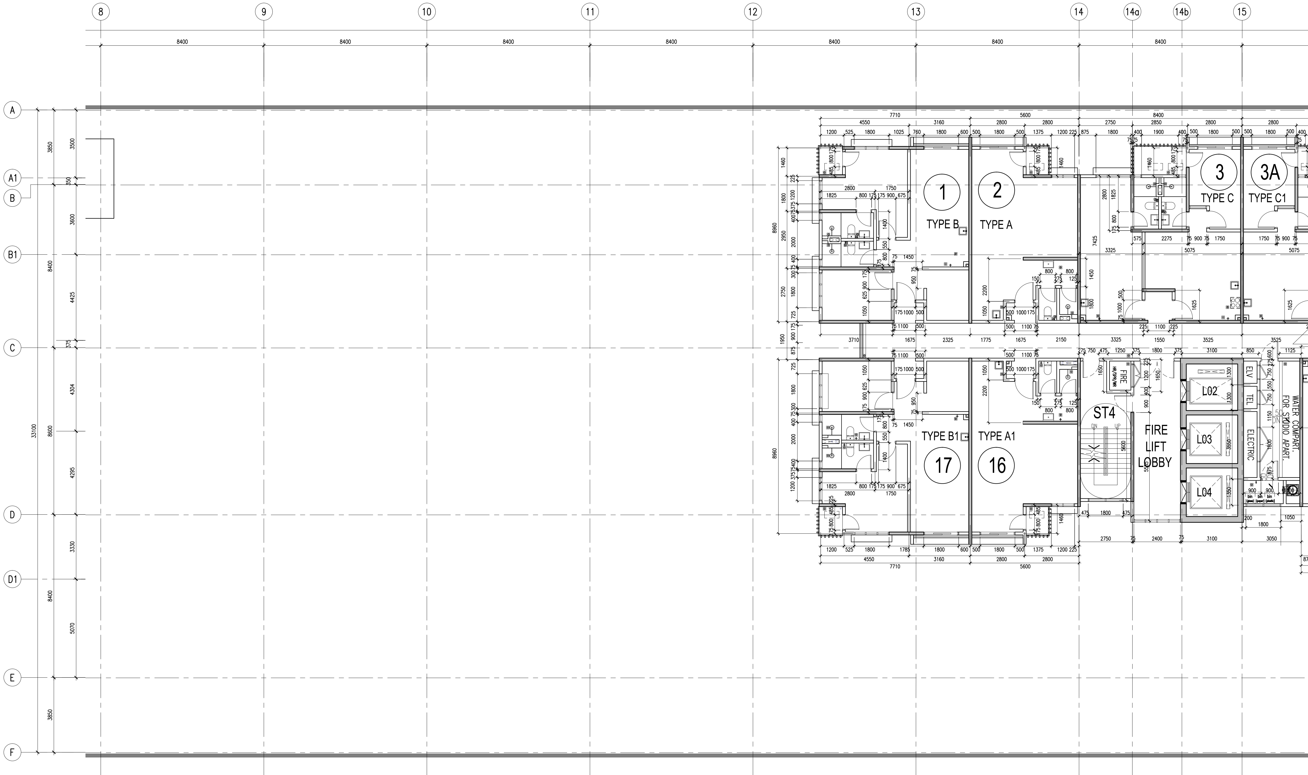
01 BRICKWALL SETTING OUT-LEVEL 10 ( PART 1 OF 4 ) 874-01 SCALE = 1 : 100
