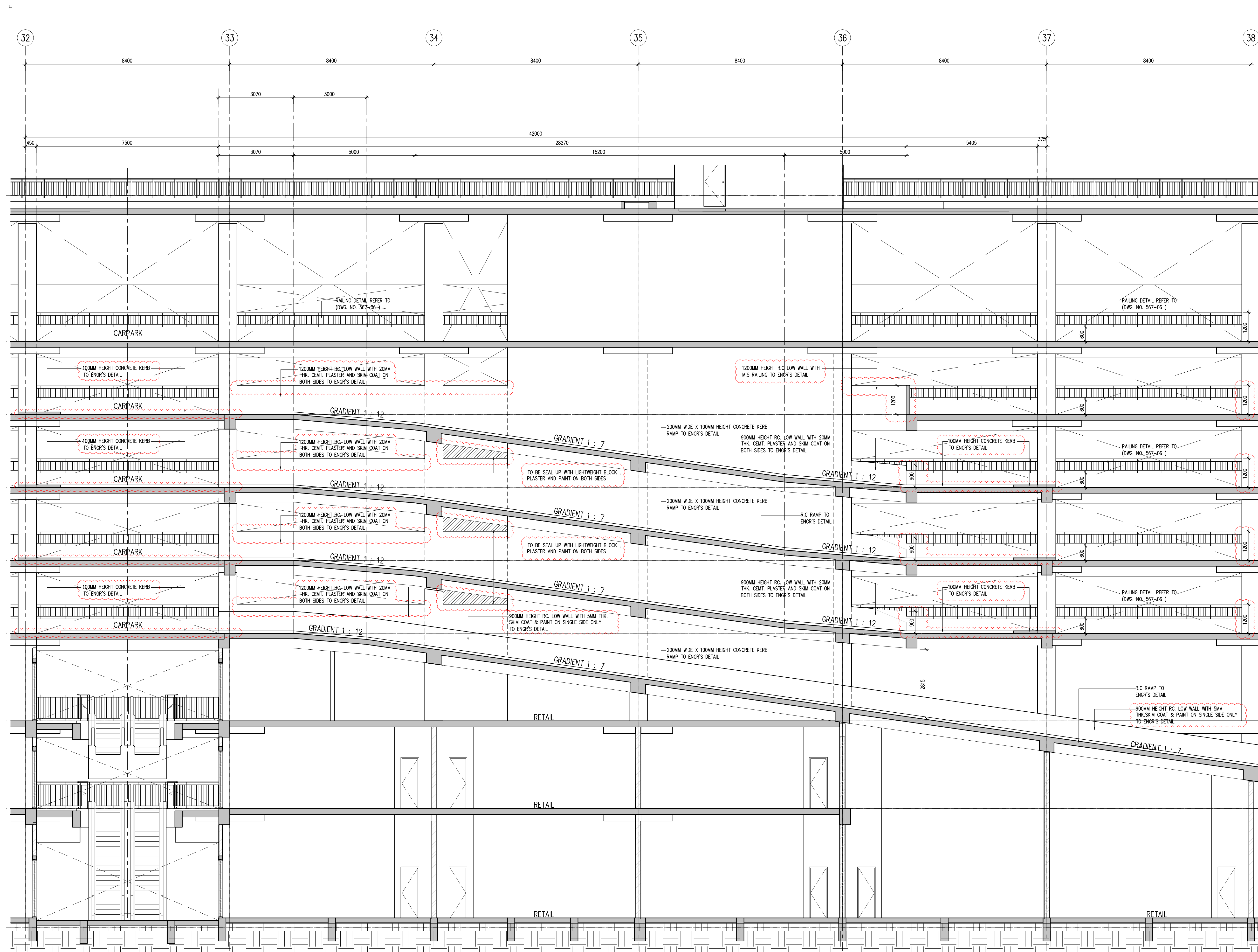
13 SECTION (2 OF 2) 523-10 SCALE = 1 : 75
