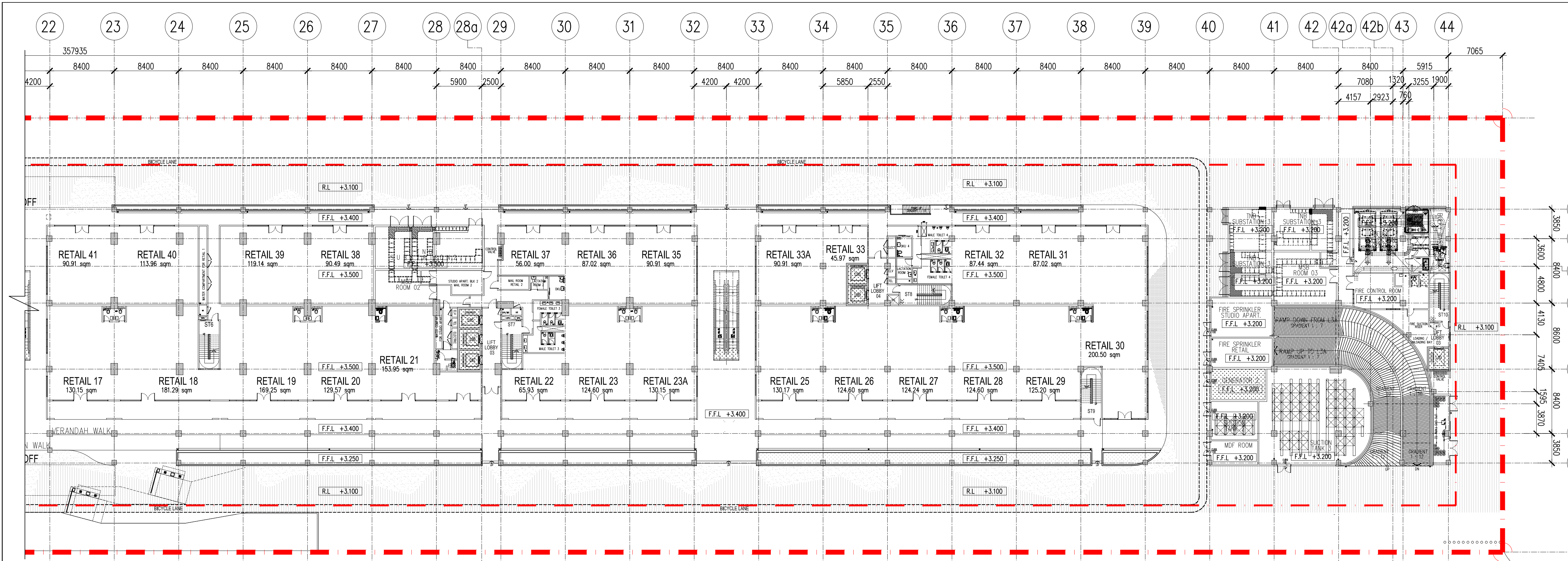
01 WATER PROOFING PLAN DEMARCATION (2 OF 2) – LEVEL 1 100 SCALE = 1 : 300
