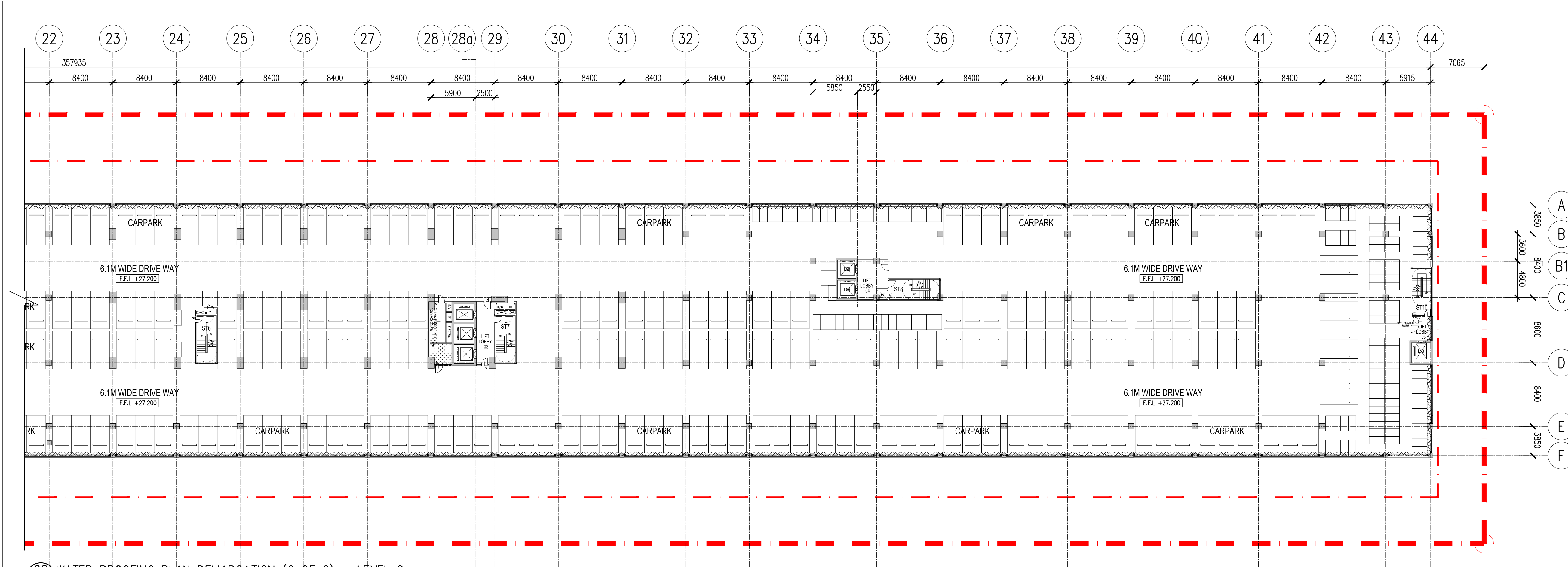
08 WATER PROOFING PLAN DEMARCATION (2 OF 2) – LEVEL 8 100 SCALE = 1 : 300
