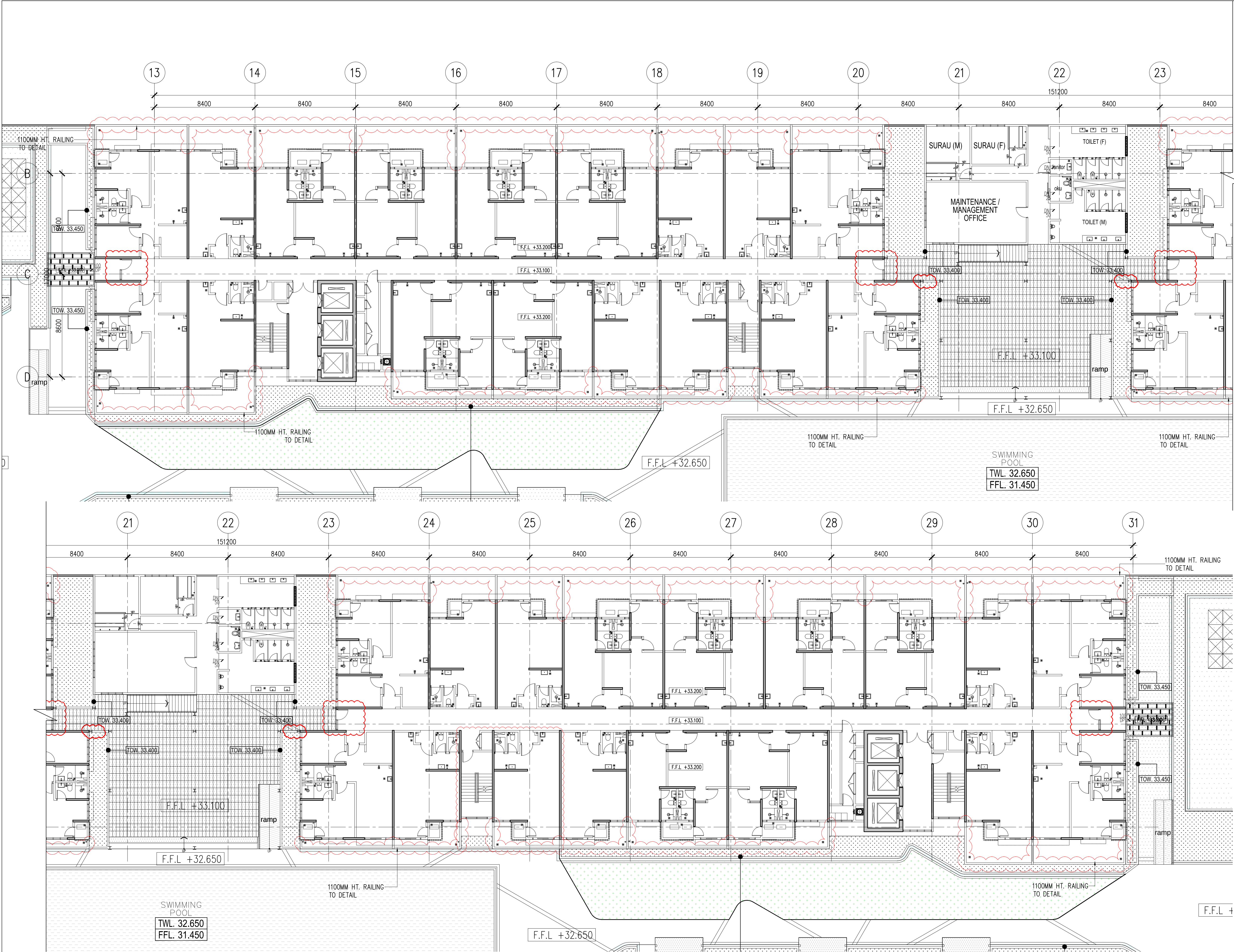
01 RAILING KEY PLAN - LEVEL 9 567-04 SCALE = 1 : 150
