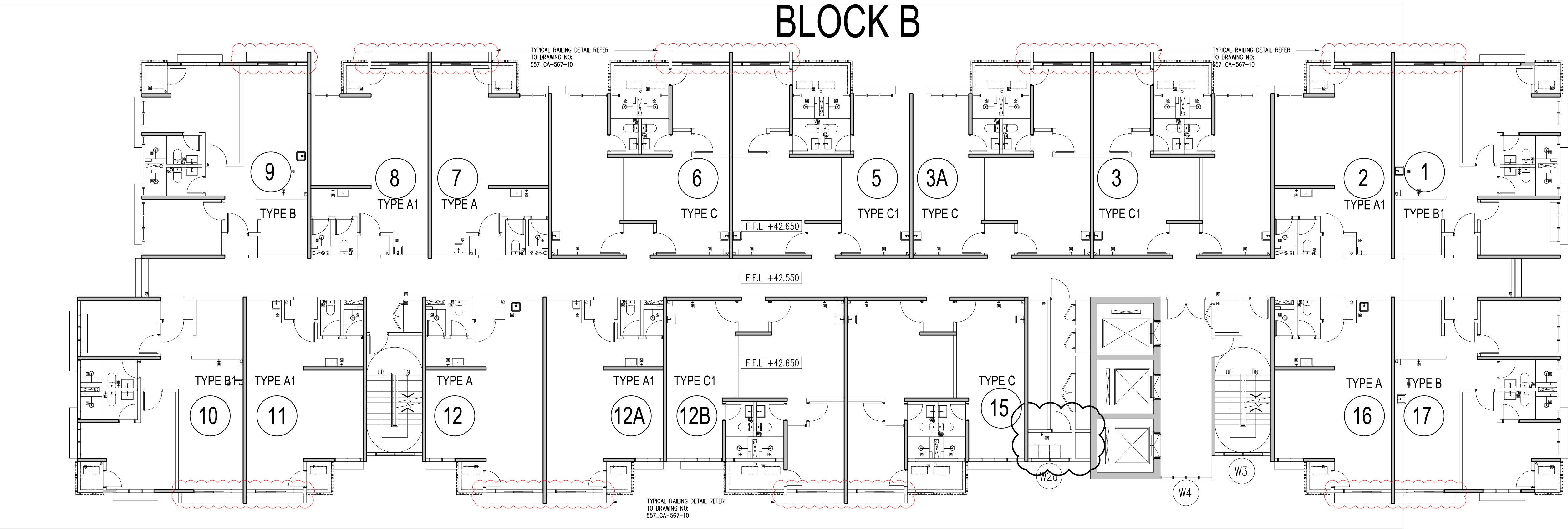
02 RAILING KEY PLAN – BLOCK B LEVEL 10–26 567–09 SCALE = 1 : NTS
