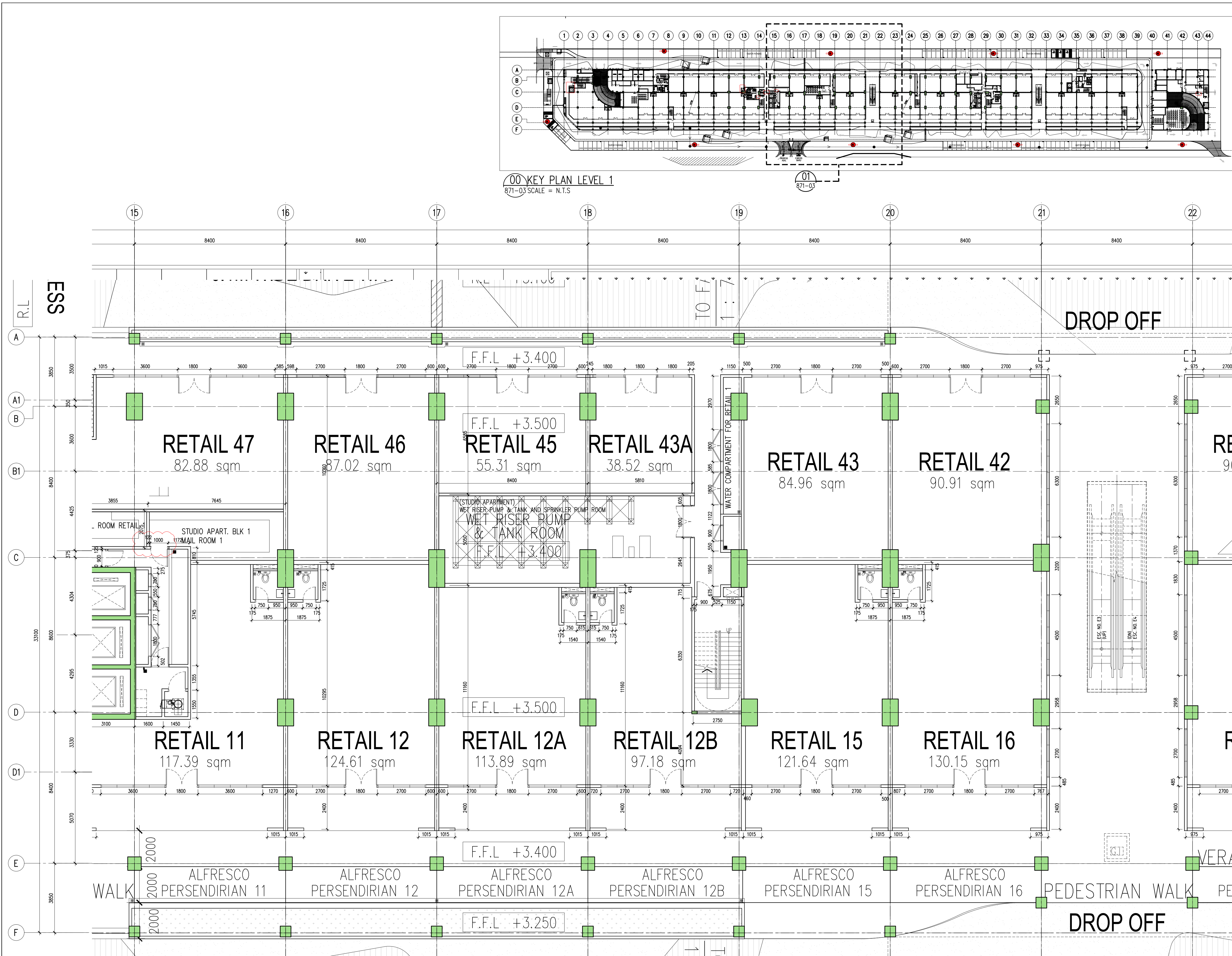
01 BRICKWALL SETTING OUT-LEVEL 1 PART 3
