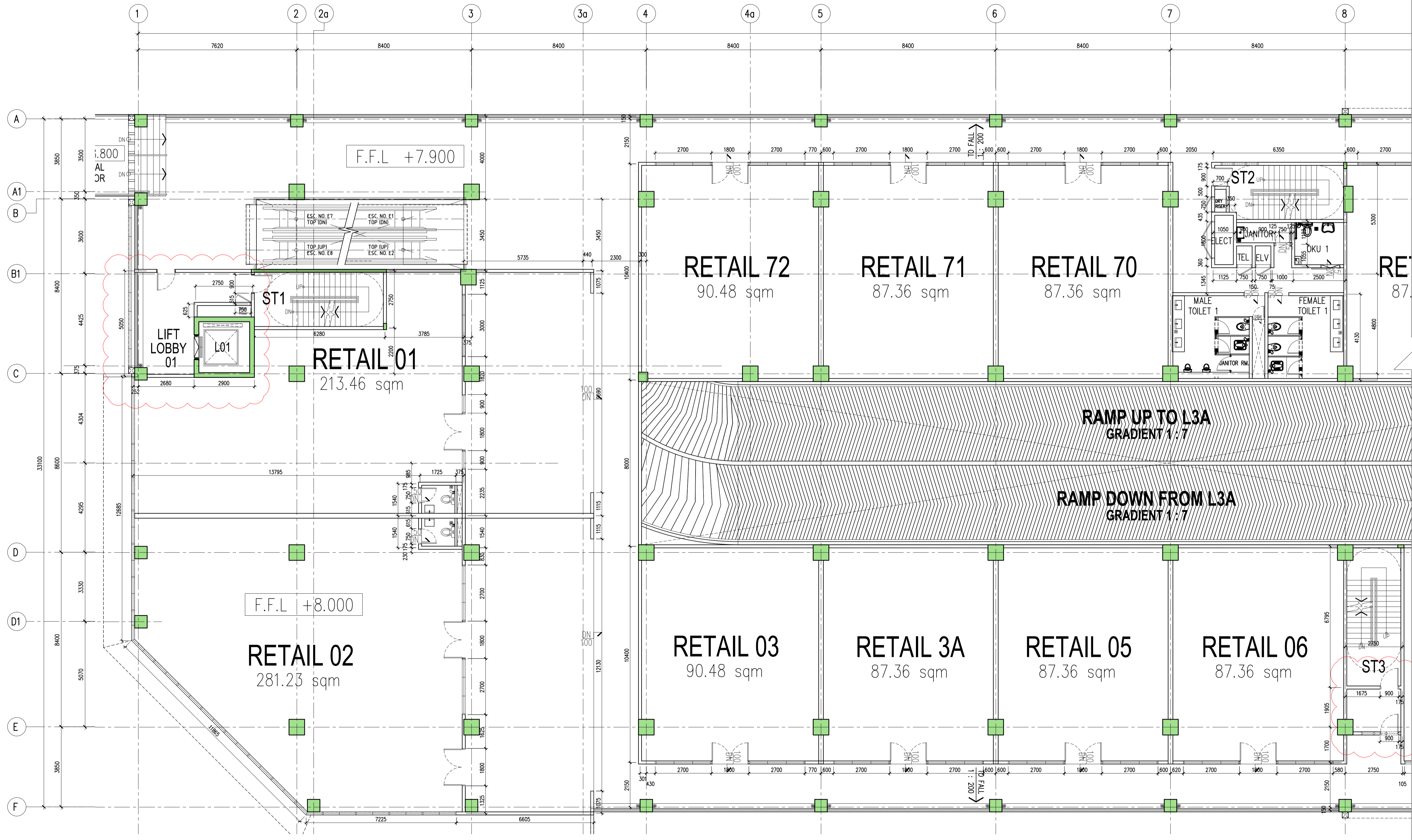
01 BRICKWALL SETTING OUT-LEVEL 2 PART 1 871-08 SCALE = 1 : 100
