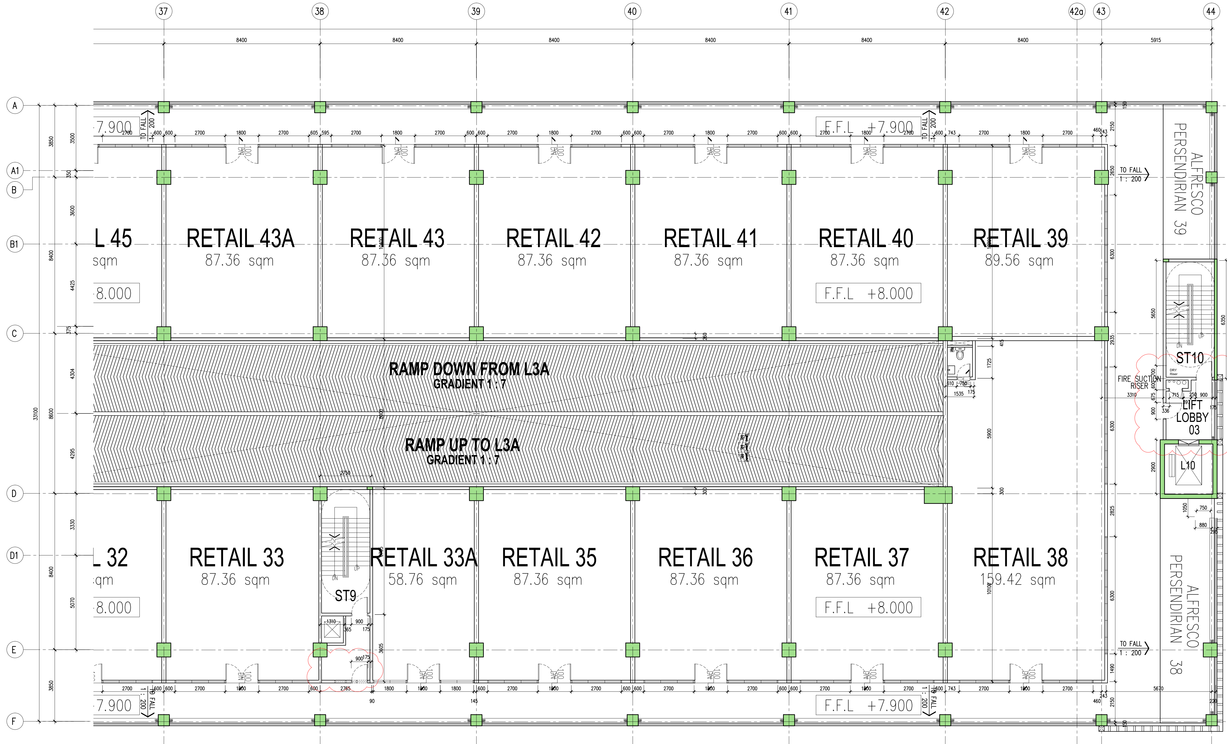
01 BRICKWALL SETTING OUT-LEVEL 2 PART 7 871-14 SCALE = 1 : 100
