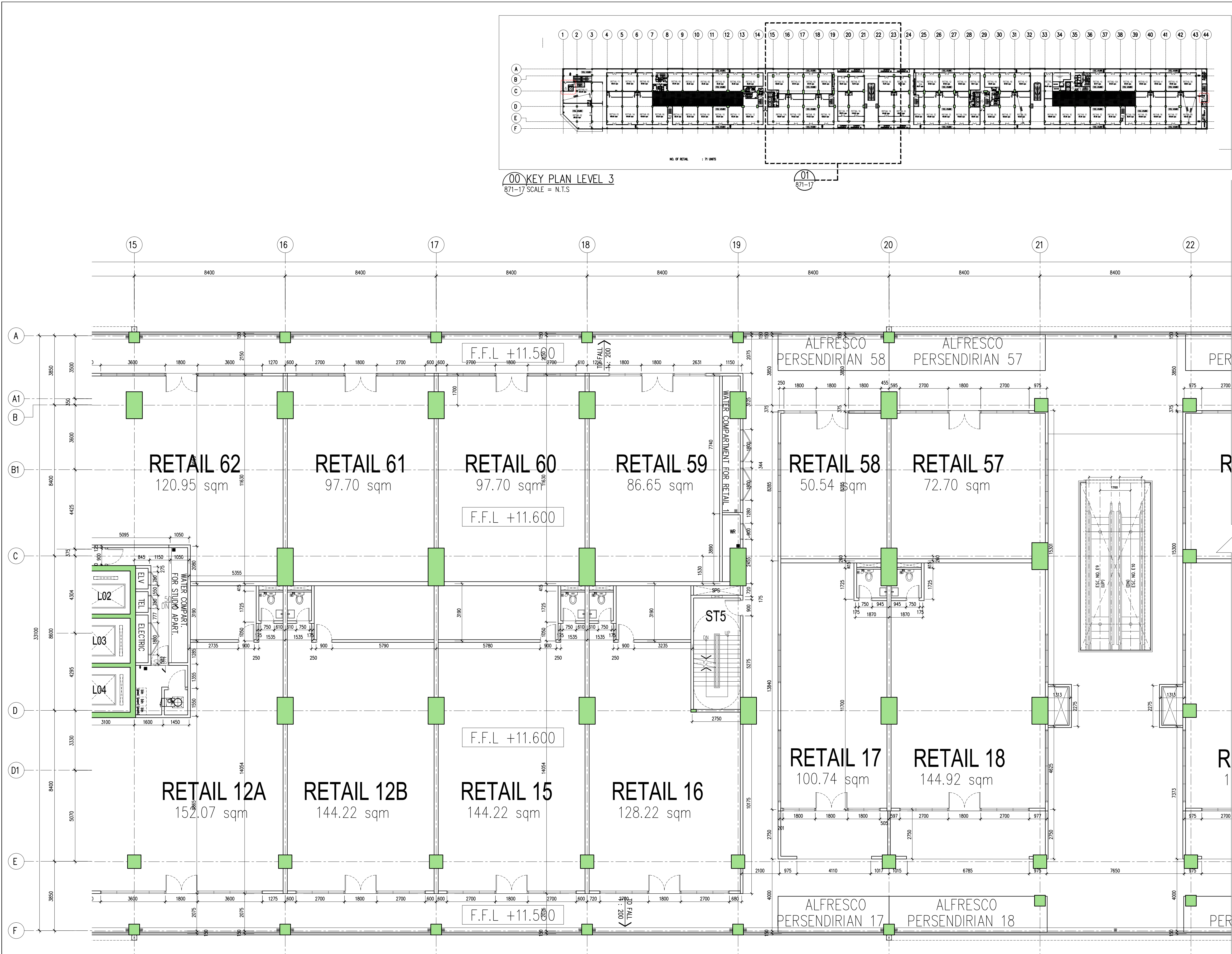
01 BRICKWALL SETTING OUT-LEVEL 3 PART 3 871-17 SCALE = 1 : 100
