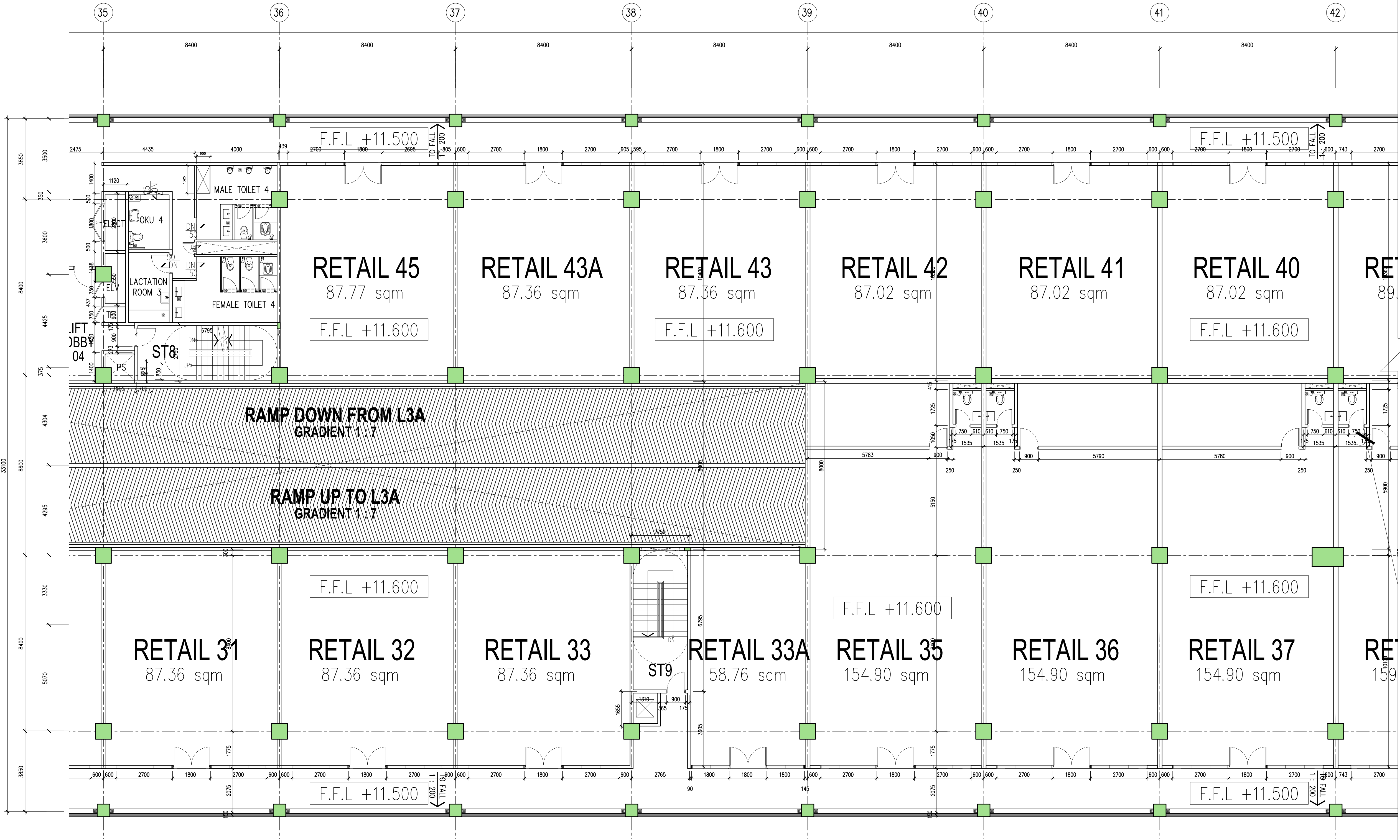
01 BRICKWALL SETTING OUT-LEVEL 3 PART 6 871-20 SCALE = 1 : 100
