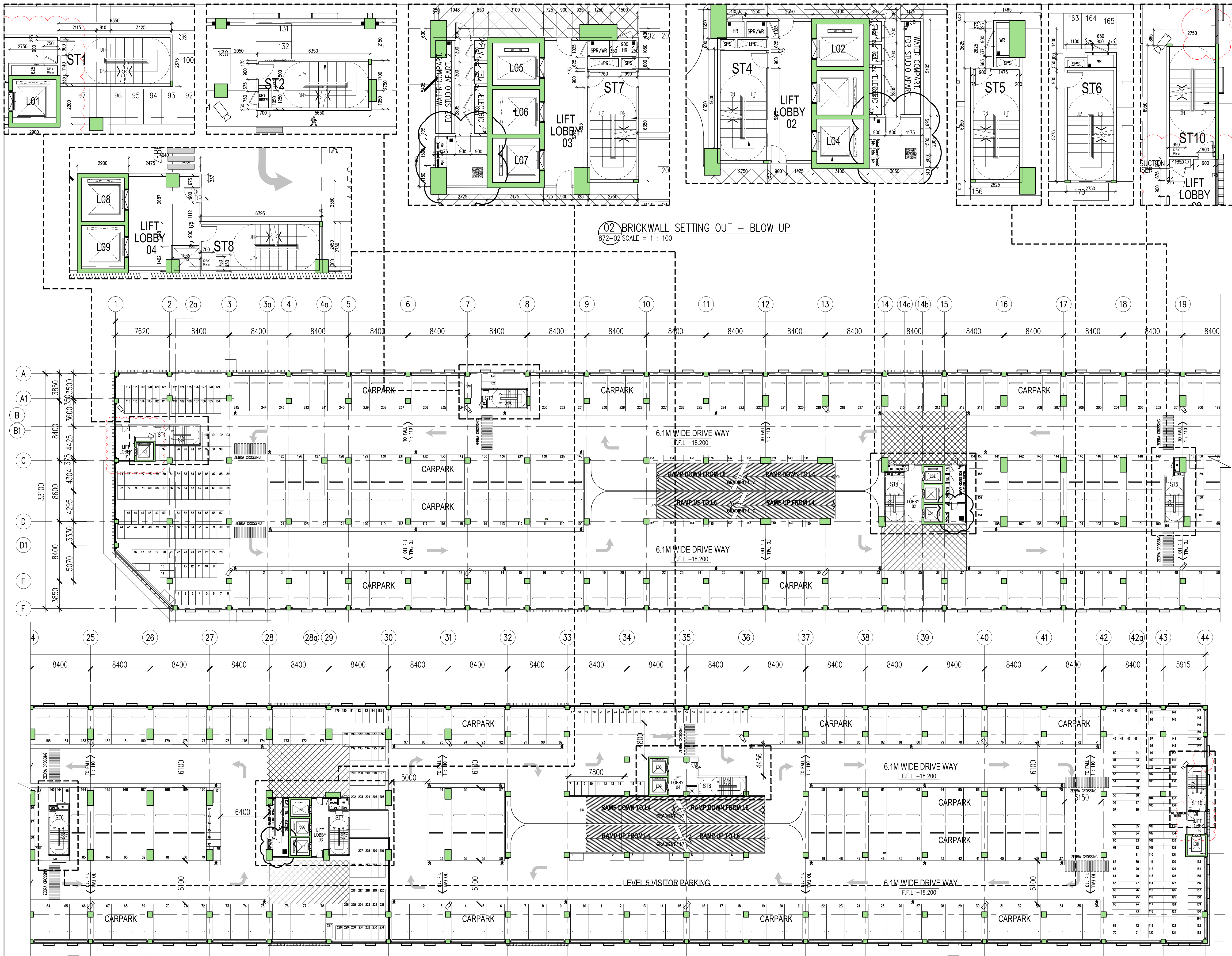
01 BRICKWALL SETTING OUT KEY PLAN - LEVEL 5-6 872-02 SCALE = 1 : 250
