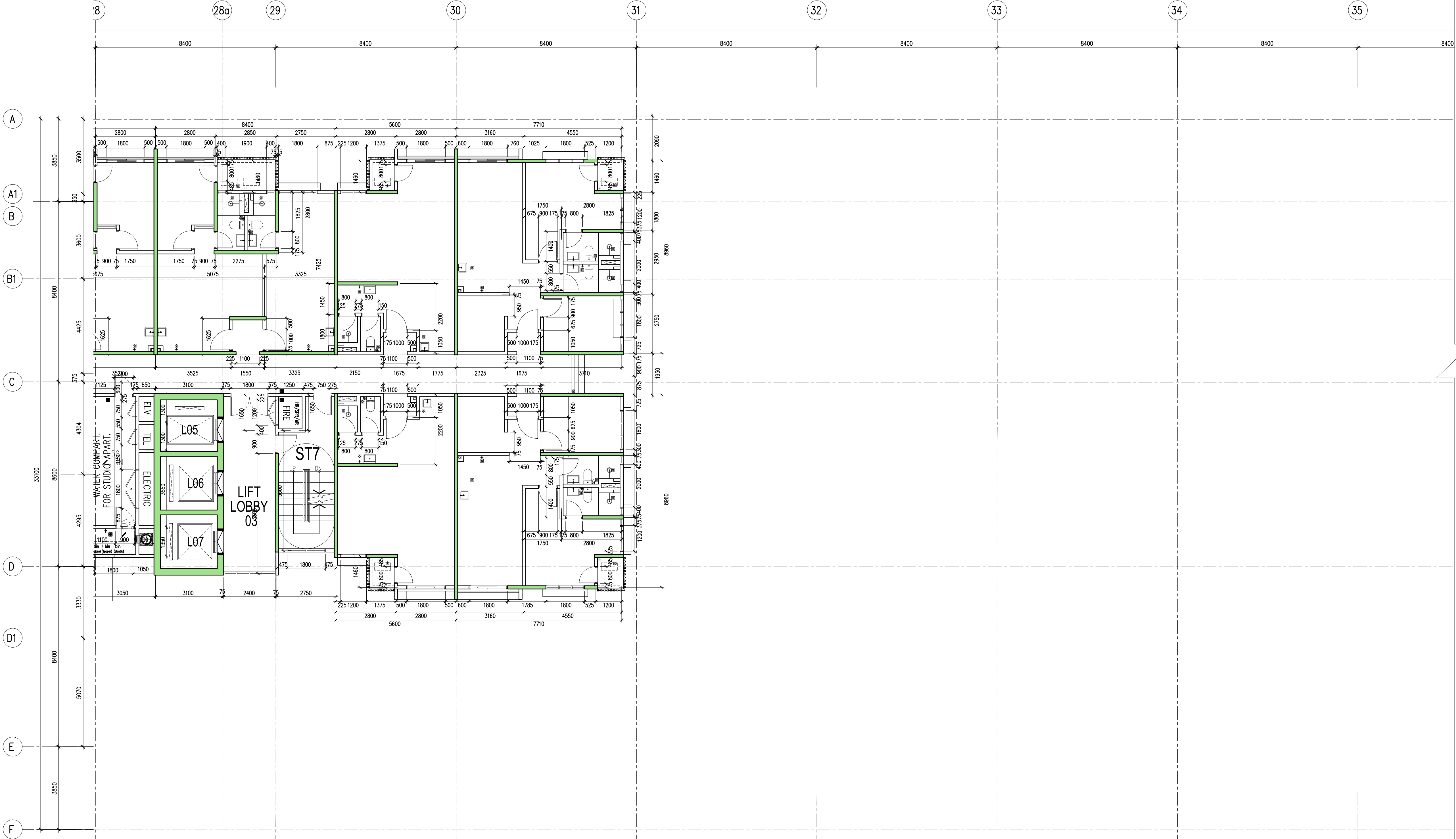
01 BRICKWALL SETTING OUT-LEVEL 11 ( PART 4 OF 4 ) 875-04 SCALE = 1 : 100
