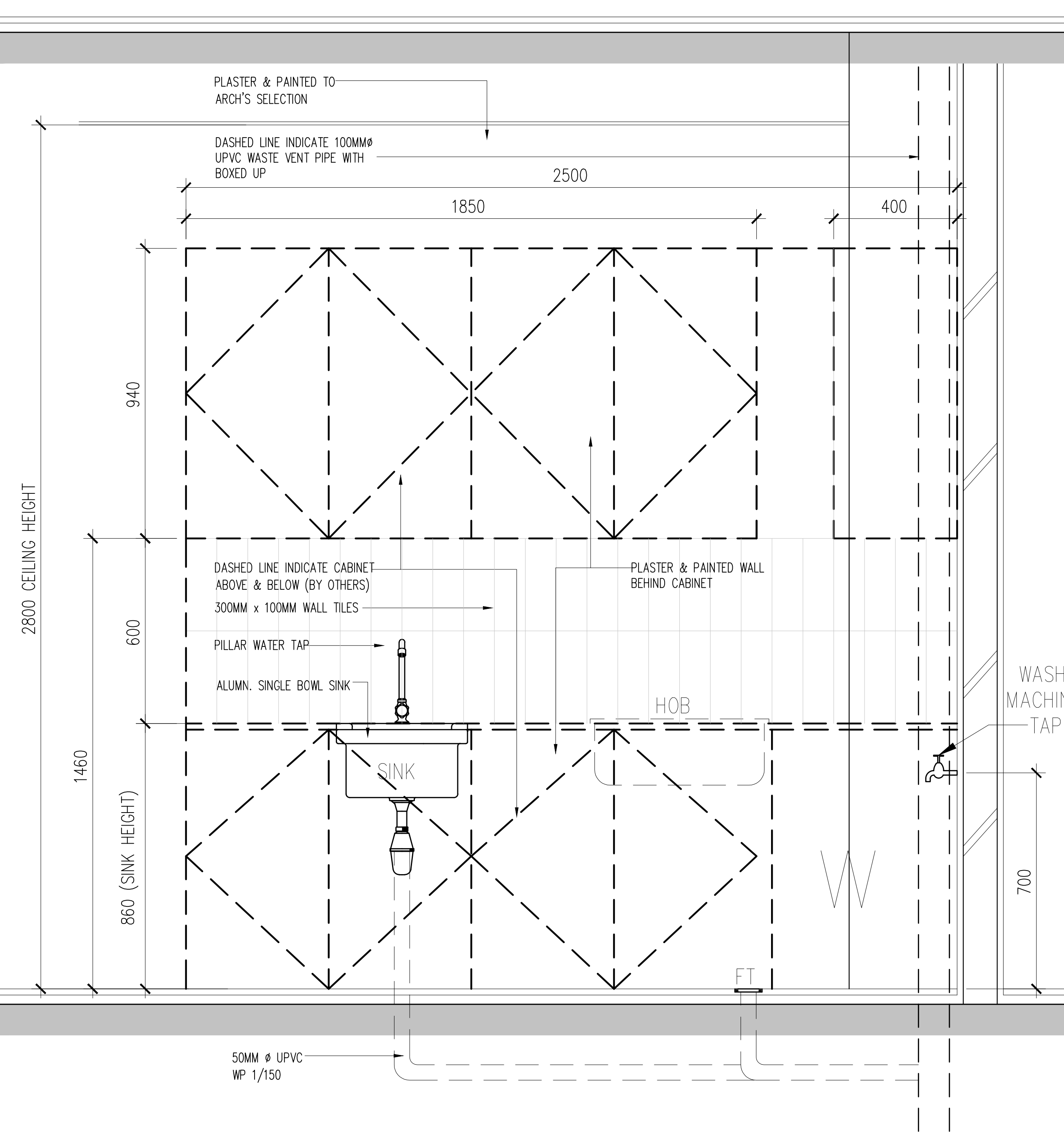
02 SECTION VIEW 'E' 910-05 SCALE = 1 : 10
