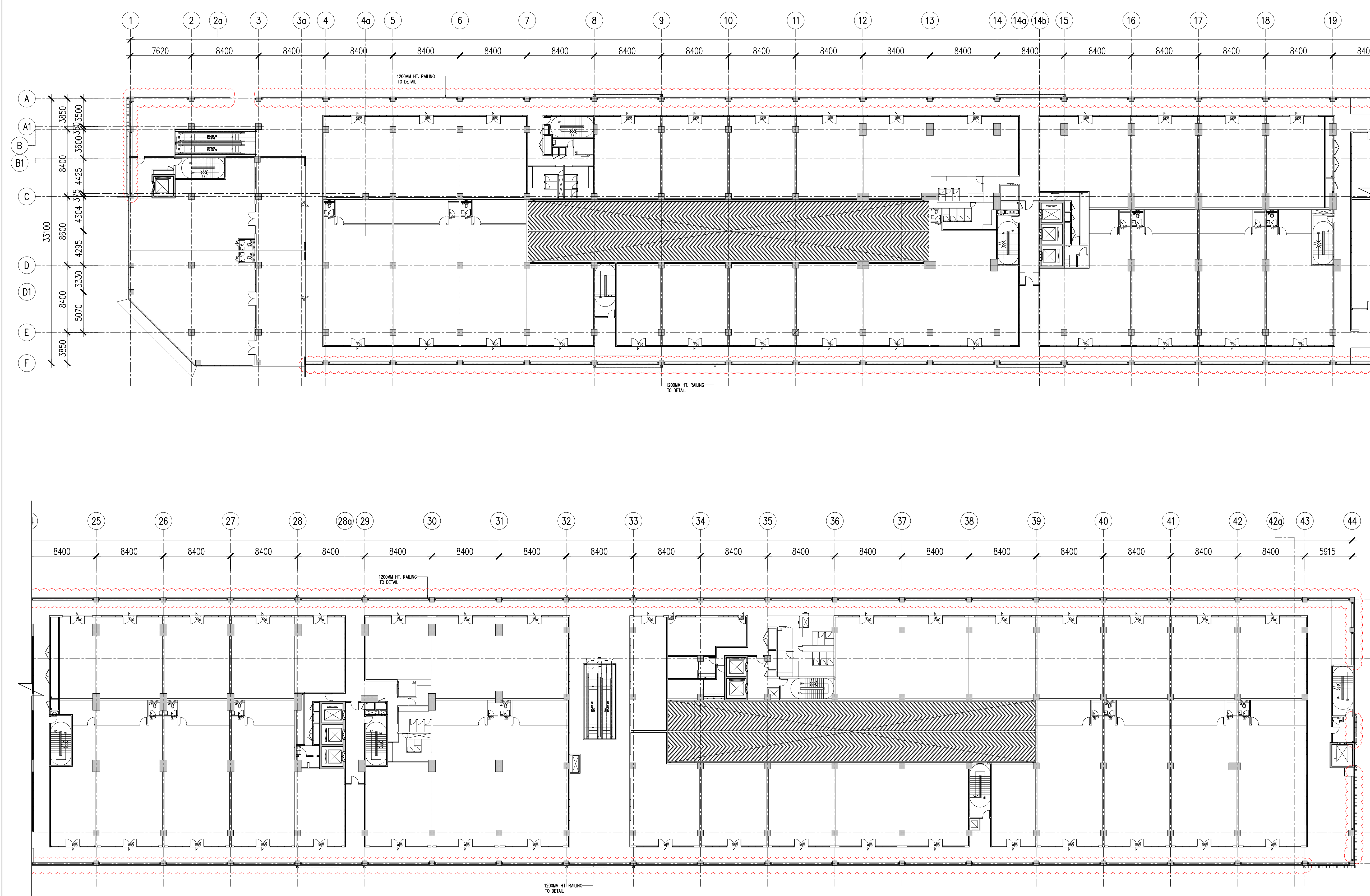
01 RAILING KEY PLAN – LEVEL 3 567-02 SCALE = 1 : 250
