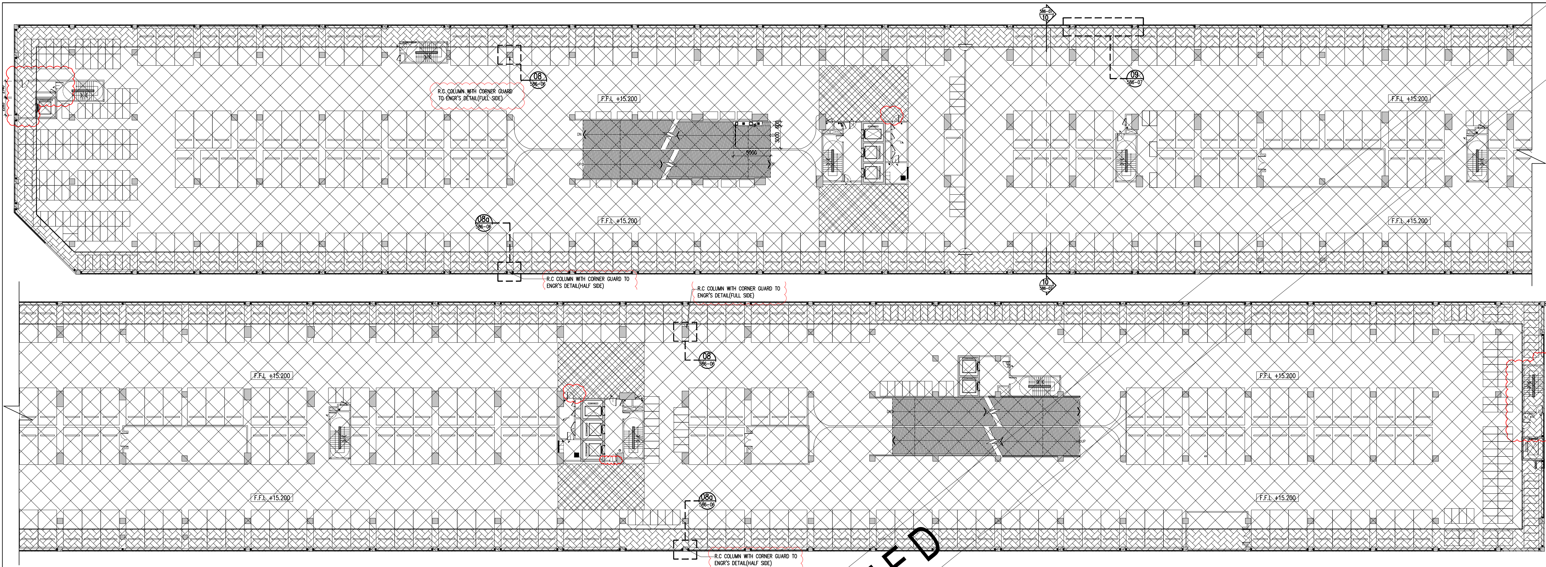
02 CARPARK DETAIL – LEVEL 4 586 SCALE = 1 : 300
