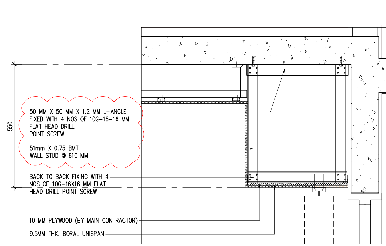
03 TYPICAL DETAIL- CURTAIN PELMET F3 710-17 SCALE = NTS
