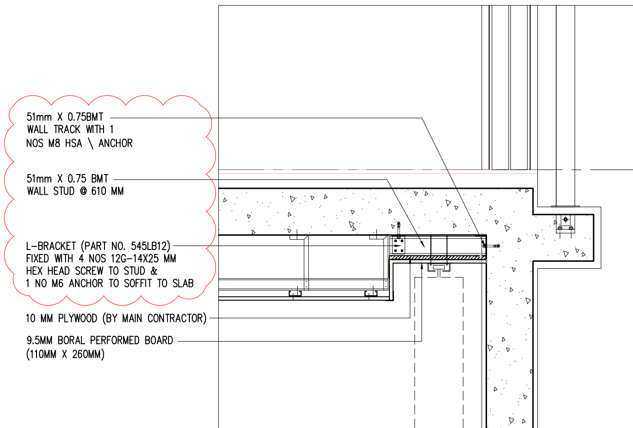
02 TYPICAL DETAIL- CURTAIN PELMET F2 710-17 SCALE = NTS
