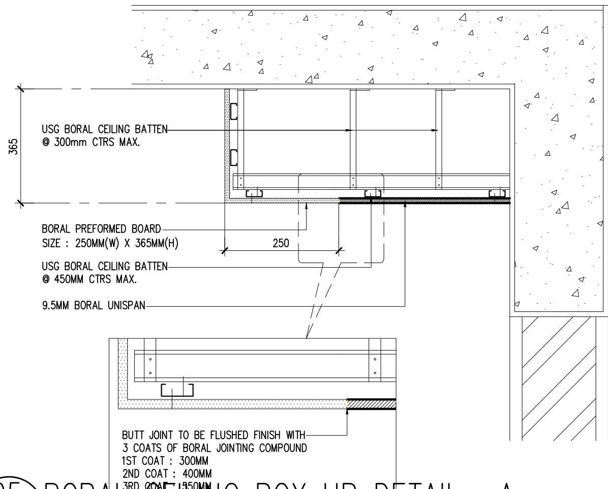
05 BORAL CEILING BOX UP DETAIL- A 710-17 SCALE = NTS (CEILING DROP 365MM)
