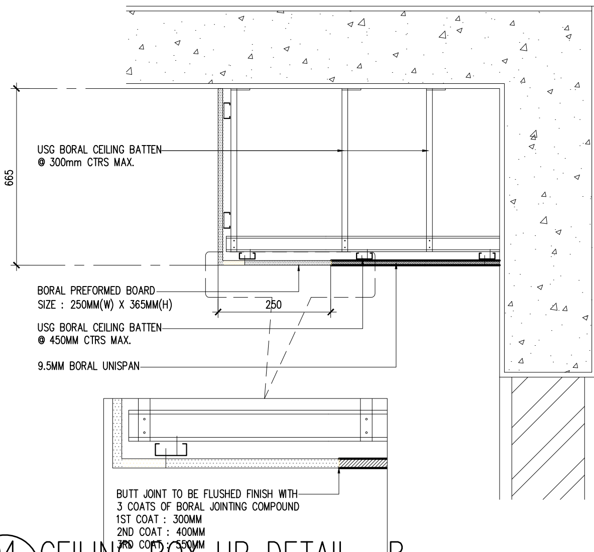
04 CEILING BOX UP DETAIL- B 710-17 SCALE = NTS (CEILING DROP 665MM)
