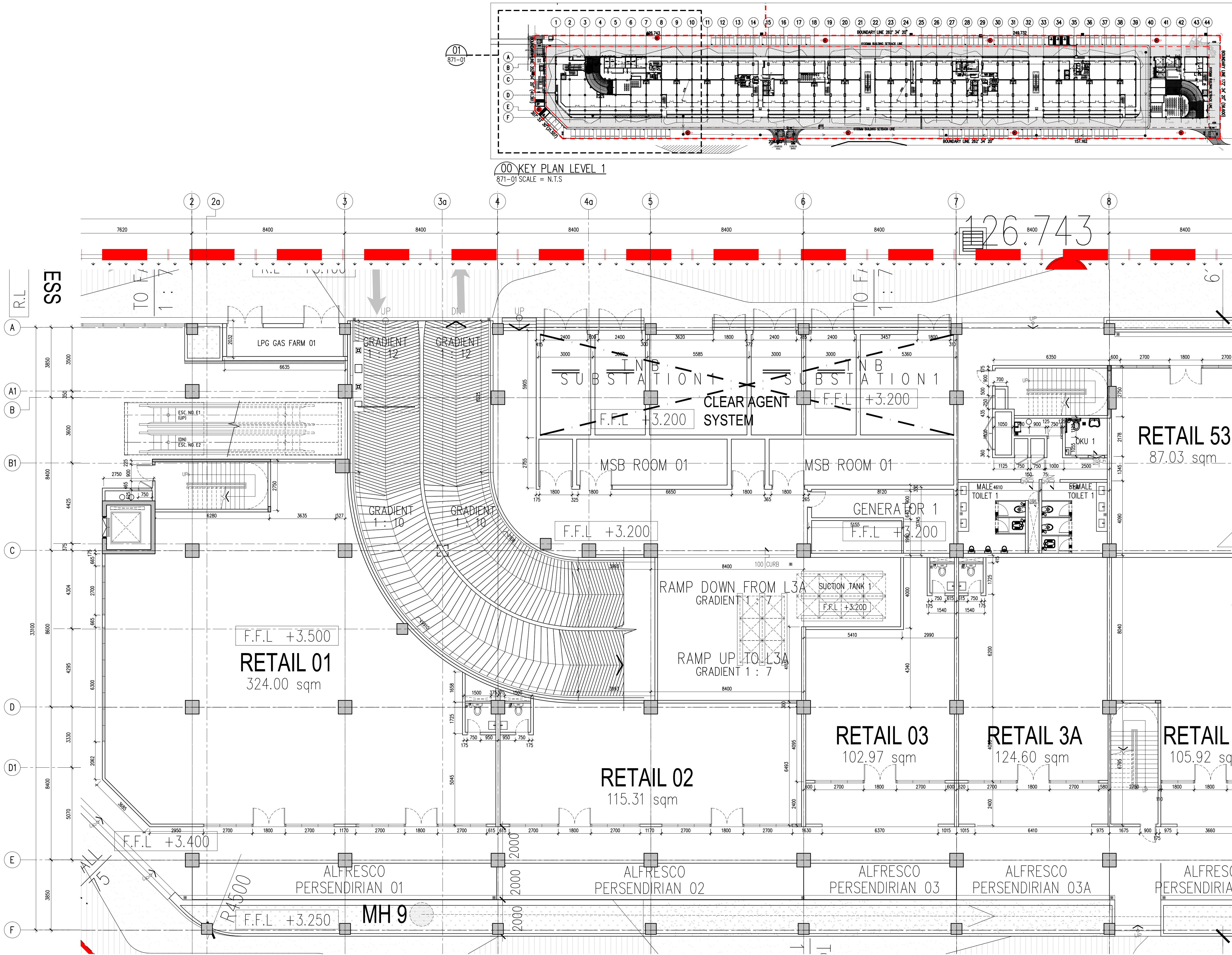
01 WALL SETTING OUT-LEVEL 1 PART 1 871-01 SCALE = 1 : 100
