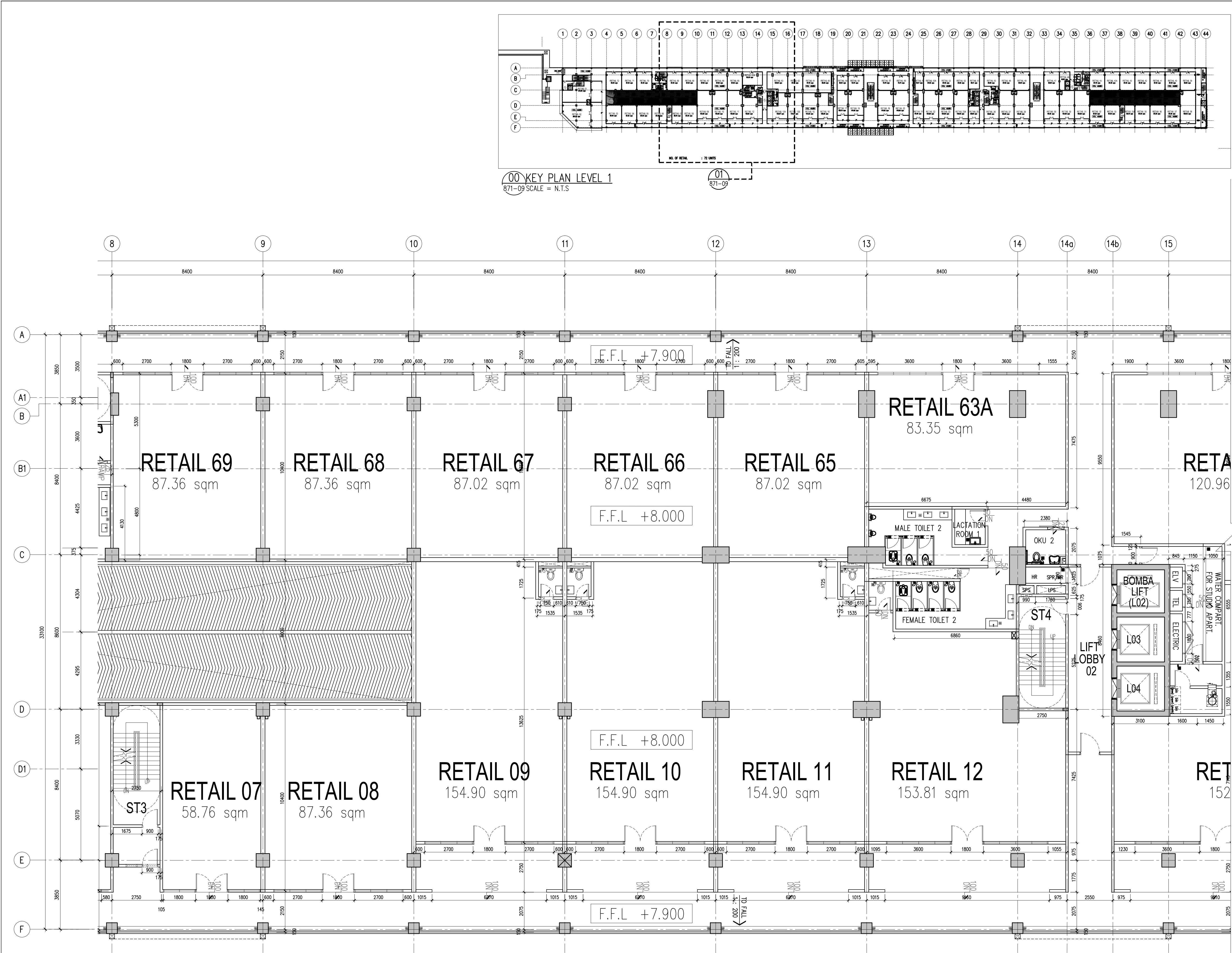
01 WALL SETTING OUT-LEVEL 2 PART 1 871-09 SCALE = 1 : 100
