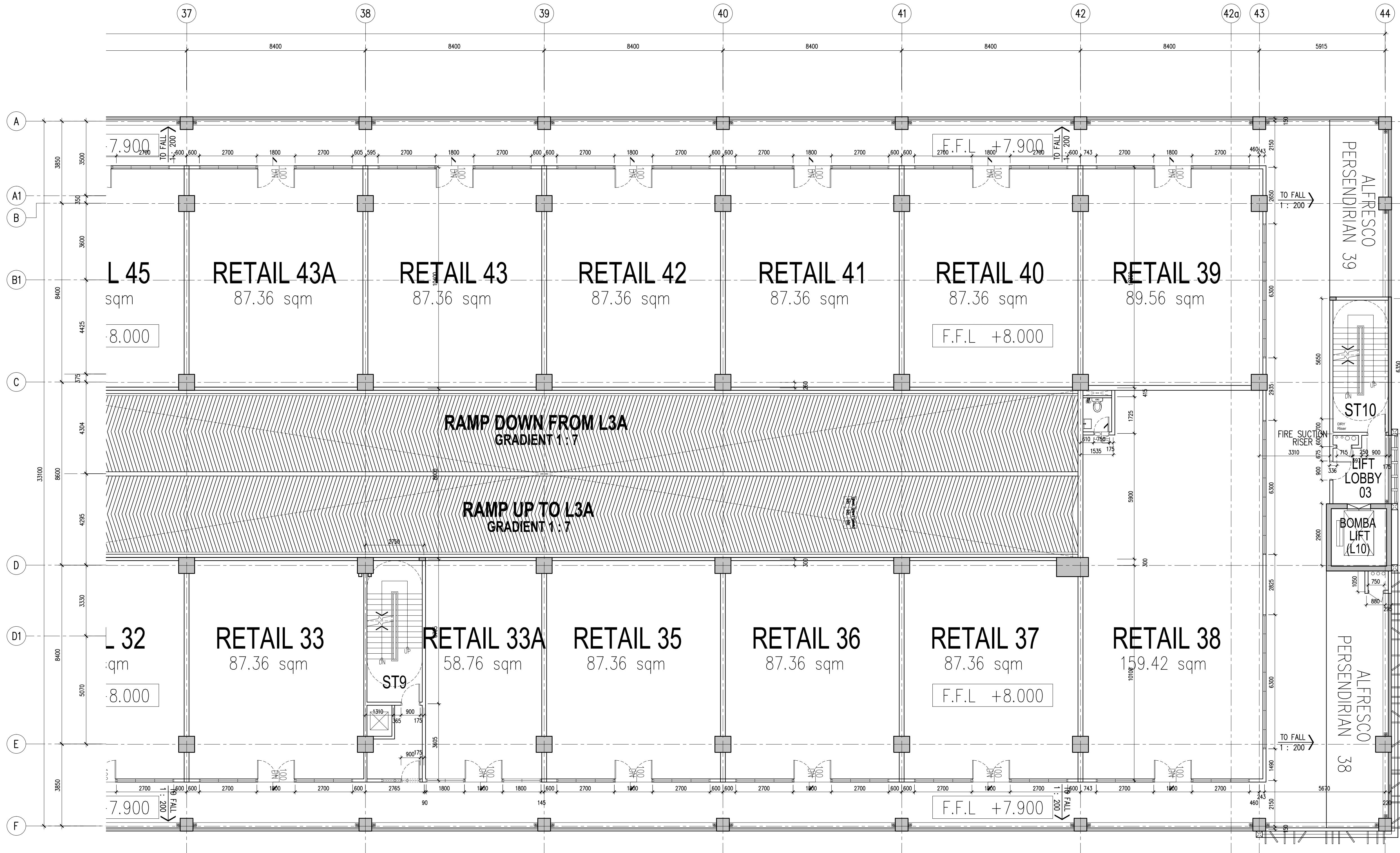
01 WALL SETTING OUT-LEVEL 2 PART 7 871-14 SCALE = 1 : 100
